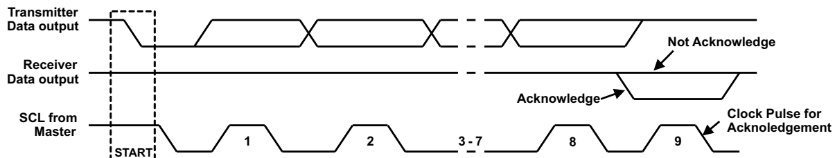
Figure 17. Acknowledge on the I 2 C Bus
