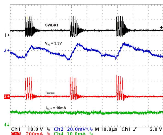
Figure 23. Buck 1 ( V_{(IO)} ) PWM Switching – Light Load
