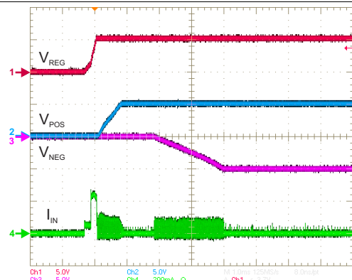
Figure 70. Inrush Current — Sequential
