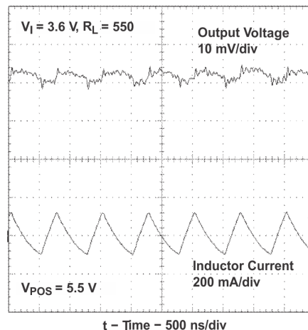
Figure 8-37. V_{POS} at Power-Save Mode Disabled
