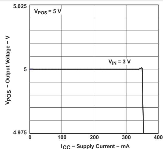
Figure 8-23. TPS65130 Output Voltage vs Output Current
