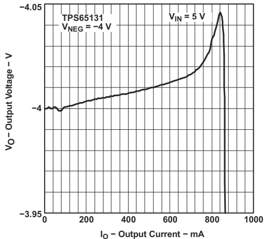
Figure 8-30. TPS65131 Output Voltage vs Output Current
