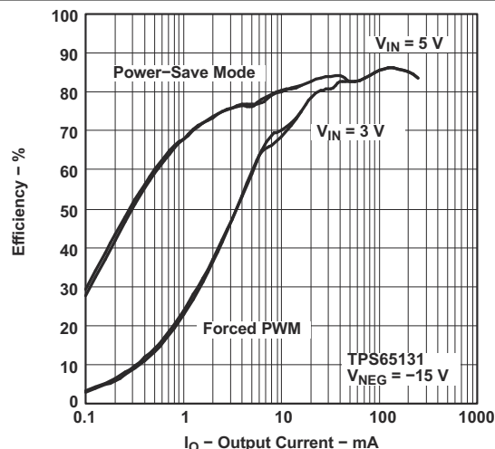
Figure 8-13. TPS65131 Efficiency vs Output Current
