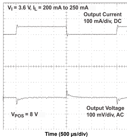
Figure 8-41. Load Transient Response
