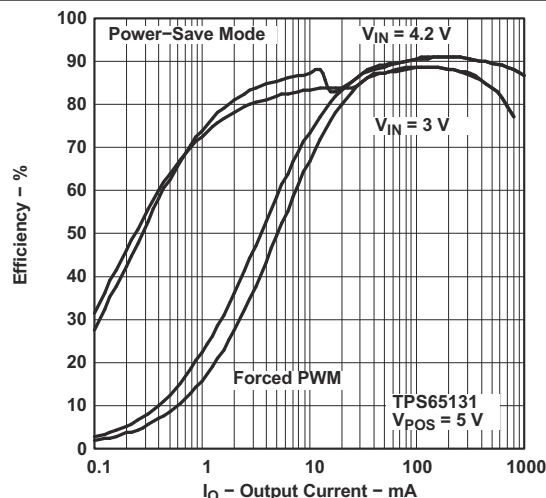
Figure 8-3. TPS65131 Efficiency vs Output Current
