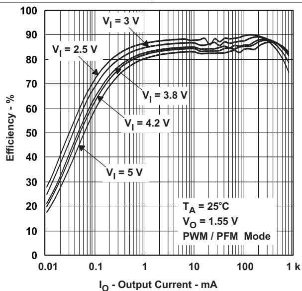
Figure 39. DCDC3 Efficiency
