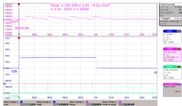
Figure 8-20. Line Transient, Light Load
