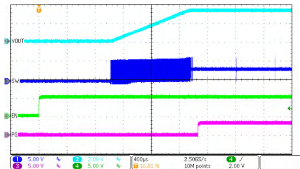
Figure 9-64. Start-Up Timing
