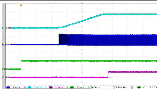
Figure 9-64. Start-Up Timing
