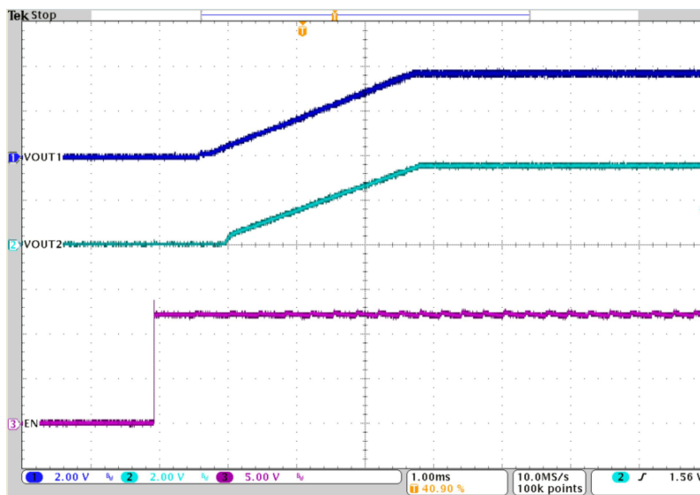
Figure 9-85. Tracking
