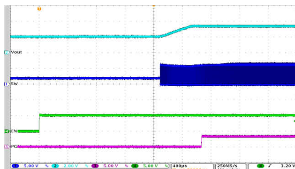
Figure 9-66. Start-Up Timing
