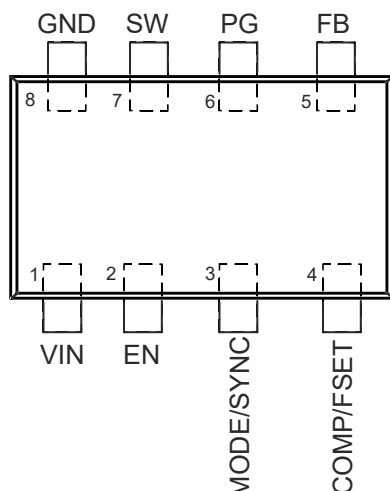
Figure 5-1. 8-Pin SOT583 DRL Package for TPS62850x-Q1 (Top View)
