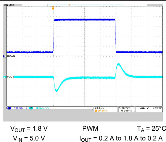
Figure 9-25. Load Transient Response
