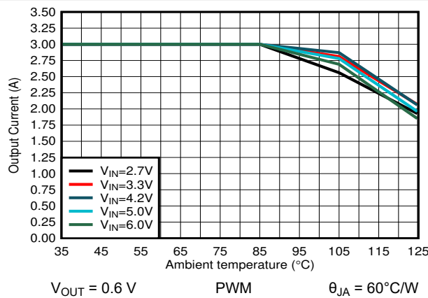
Figure 9-18. Output Current vs Ambient Temperature
