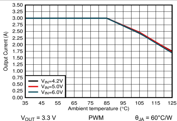
Figure 9-21. Output Current vs Ambient Temperature
