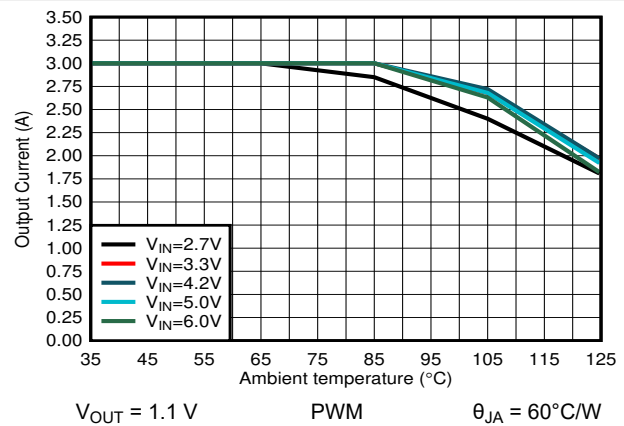
Figure 9-19. Output Current vs Ambient Temperature
