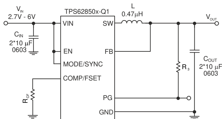
Figure 9-57. Schematic for Fixed Output Voltage Versions
