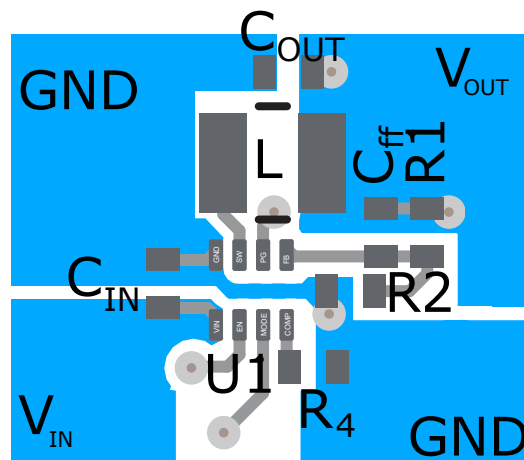
Figure 9-61. Example Layout
