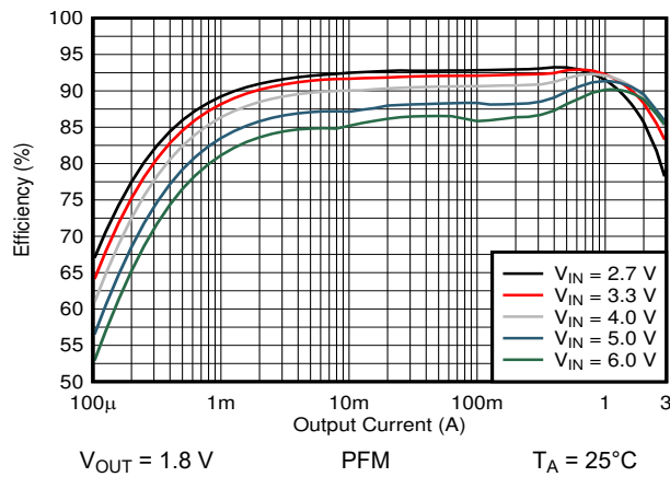
Figure 9-4. Efficiency vs Output Current
