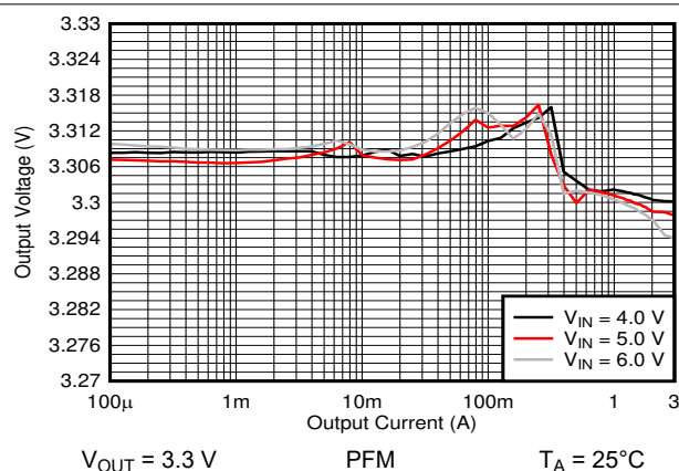
Figure 9-10. Output Voltage vs Output Current
