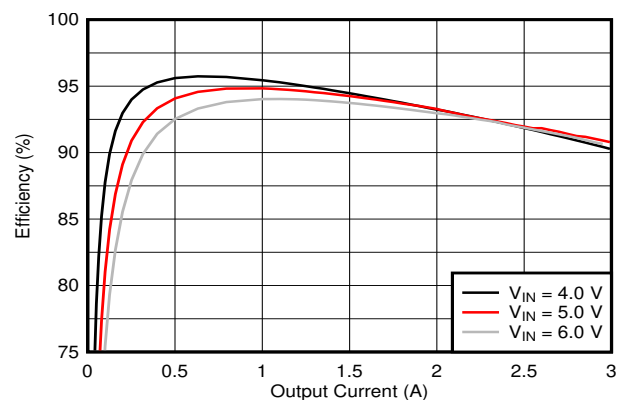
Efficiency vs I_{OUT} , V_{OUT} = 3.3\text{V}
