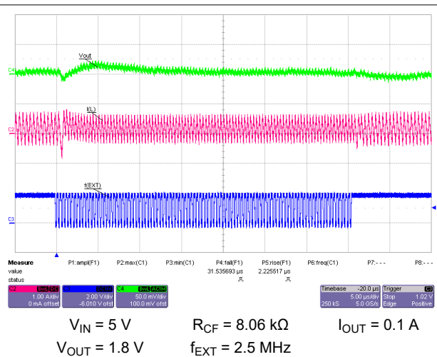
Figure 9-60. Switching from External Synchronization to Internal Fixed Frequency
