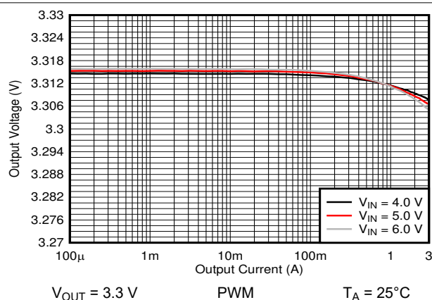
Figure 9-11. Output Voltage vs Output Current
