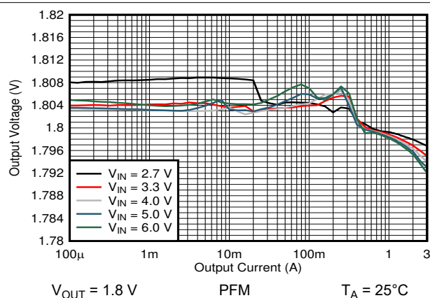
Figure 9-12. Output Voltage vs Output Current
