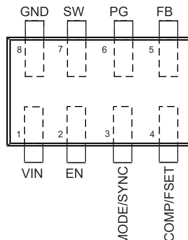
Figure 5-2. 8-Pin SOT583 DYC Package for TPS62850x-Q1 (Top View)
