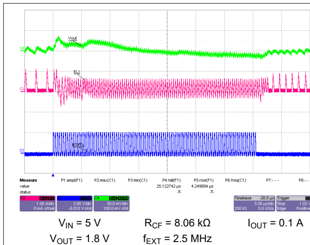
Figure 9-59. Switching from External Synchronization to Power-Save Mode (PFM)
