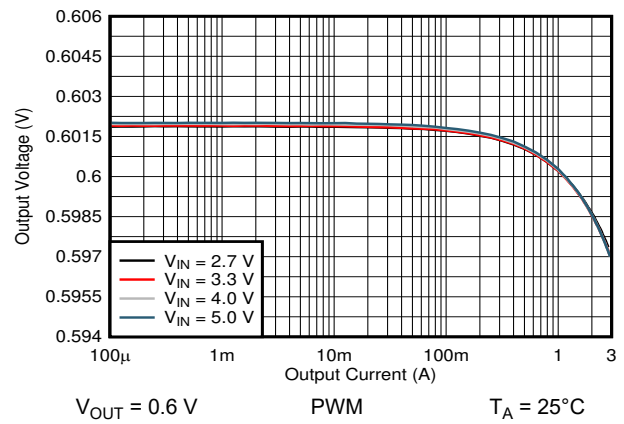
Figure 9-17. Output Voltage vs Output Current
