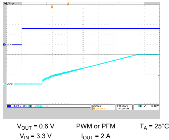
Figure 9-56. Start-Up Timing
