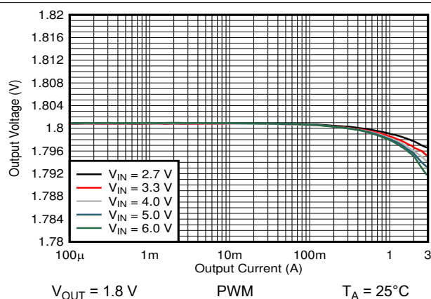
Figure 9-13. Output Voltage vs Output Current
