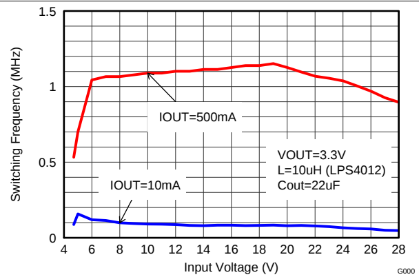
Figure 28. Switching Frequency
