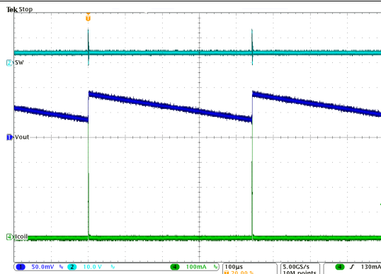
Figure 47. Typical Operation in Sleep Mode, I_{OUT}=1\text{ mA}
