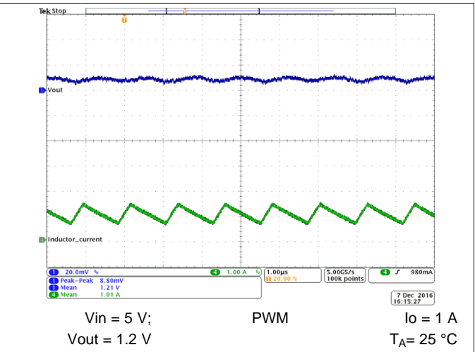
Figure 37. Output Voltage Ripple
