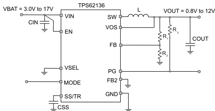
Figure 3. Measurement Setup
