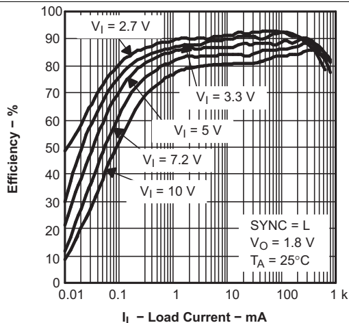
Figure 21. TPS62054 Efficiency vs Load Current in PFM Mode
