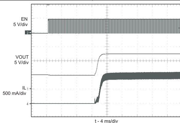
Figure 10. Analog Dimming Start-up
