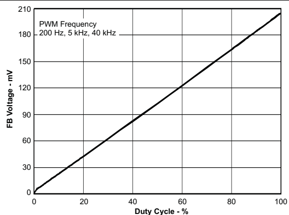
Figure 9. Analog Dimming Linearity
