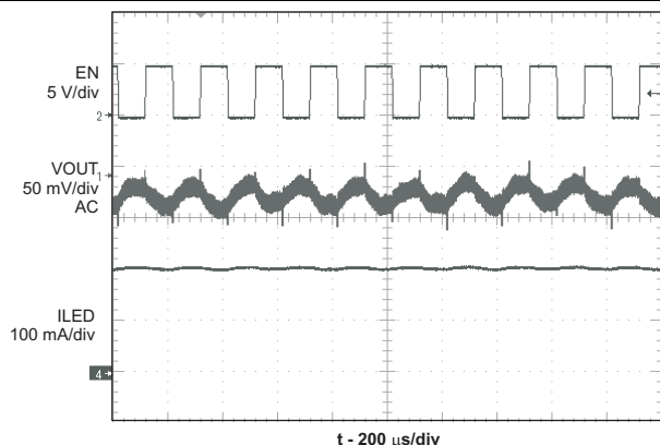
Figure 8. Analog Dimming
