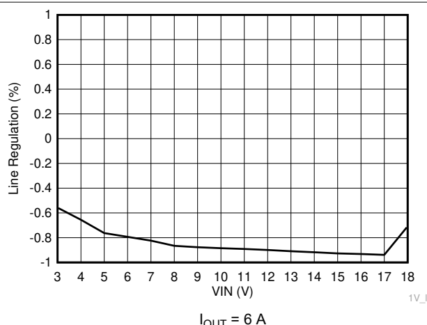
Figure 7-11. Line Regulation
