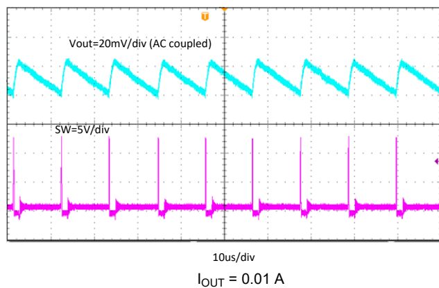
Figure 7-12. TPS566231 Output Voltage Ripple
