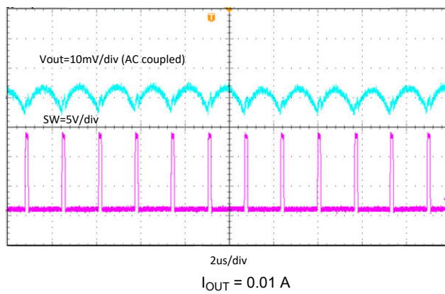
Figure 7-13. TPS566238 Output Voltage Ripple
