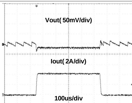
Figure 9. 1.05 V Load Transient Response
