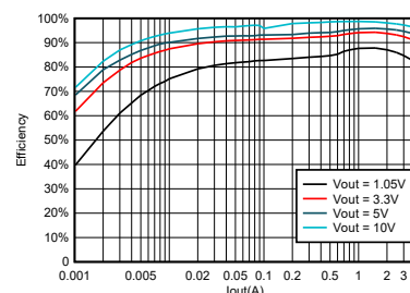
TPS564252B Efficiency at V_{IN} = 12V
