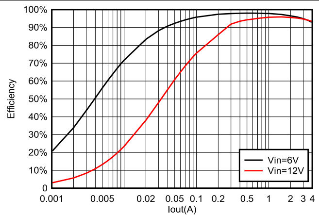
Figure 5-20. TPS564257B Efficiency at 5 V_{OUT} With a 4.7 \mu\text{H} Inductor
