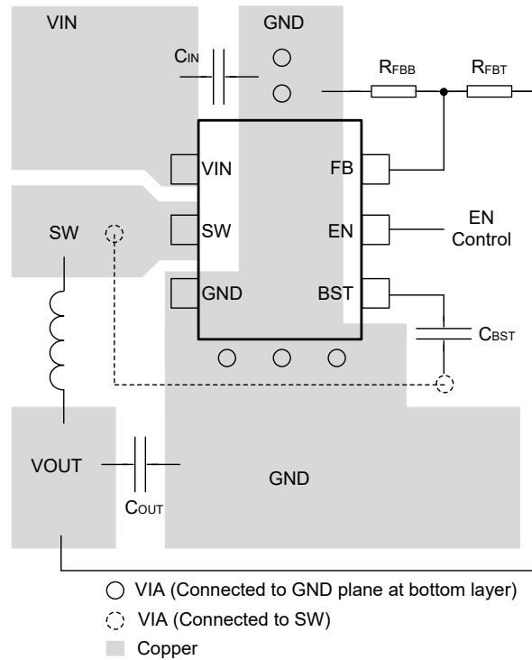
Figure 7-26. Suggested Layout
