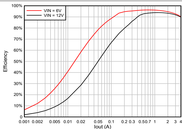
Figure 5-26. TPS564257C Efficiency at 3.3\text{V}_{OUT} With a 2.2\mu\text{H} Inductor
