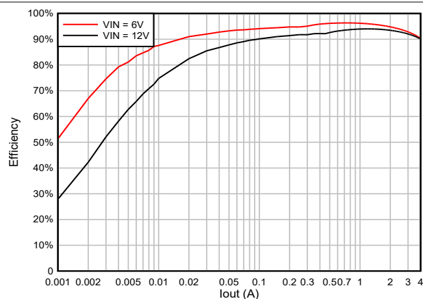
Figure 5-25. TPS564252C Efficiency at 3.3\text{V}_{OUT} With a 2.2\mu\text{H} Inductor
