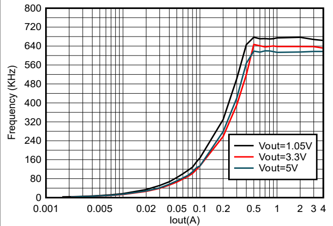
Figure 5-10. TPS564252B Frequency vs Loading, V_{IN} = 12\text{V}
