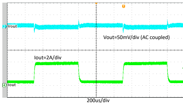
Figure 7-15. TPS564252B Transient Response With 0.4A to 3.6A
