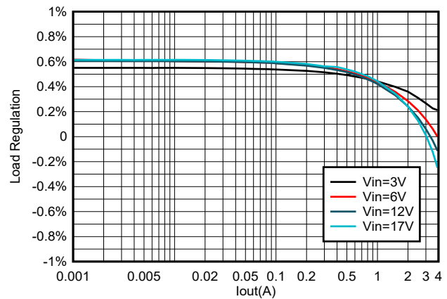
Figure 7-5. TPS564252B Load Regulation vs Loading
