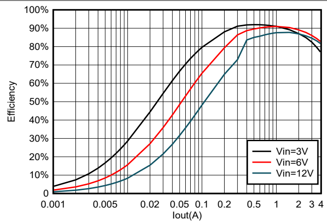
Figure 5-14. TPS564257B Efficiency at 1.05 V_{OUT} With a 1.5 \mu\text{H} Inductor
