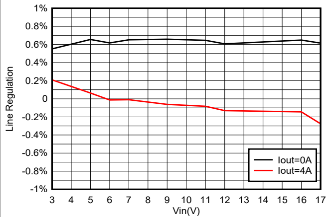
Figure 7-9. TPS564257B Line Regulation vs V_{IN}
