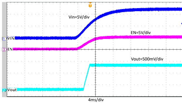
Figure 7-20. Start-up With V_{IN} Rising, I_{OUT} = 4A
