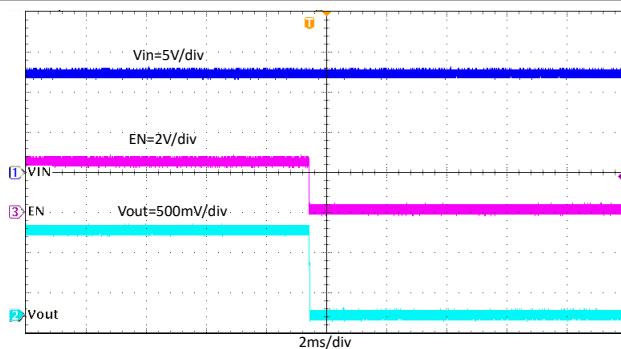
Figure 7-19. Shutdown Through EN, I_{OUT} = 4A
