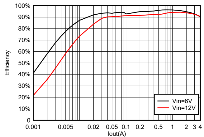
Figure 5-18. TPS564255B Efficiency at 3.3 V_{OUT} With a 3.3 \mu\text{H} Inductor
