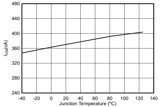
Figure 5-2. TPS564257B, TPS564257C Quiescent Current
