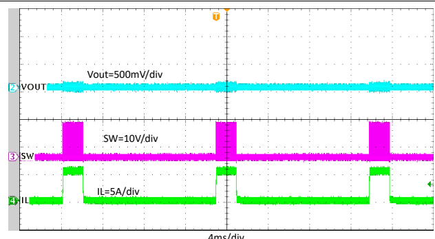
Figure 7-25. Output Hard Short Hiccup
