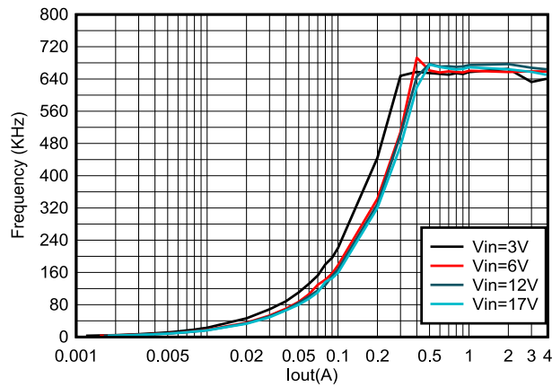
Figure 7-2. TPS564252B Frequency vs Loading
