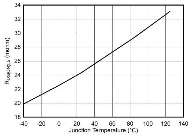
Figure 5-6. Low-Side R_{DS(ON)}
