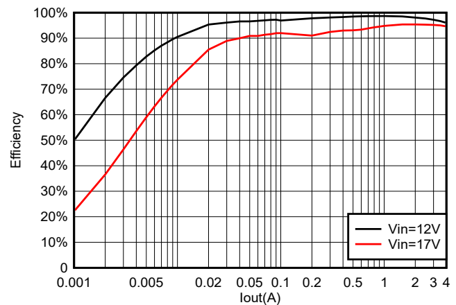
Figure 5-24. TPS564255B Efficiency at 10 V_{OUT} With a 6.8 \mu\text{H} Inductor
