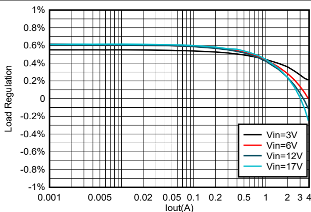
Figure 7-6. TPS564257B Load Regulation vs Loading
