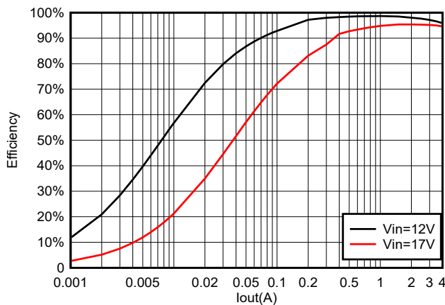
Figure 5-23. TPS564257B Efficiency at 10 V_{OUT} With a 6.8 \mu\text{H} Inductor
