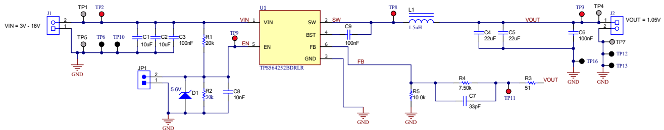
Figure 7-1. Schematic
