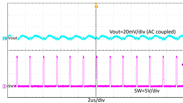
Figure 7-12. TPS564257B Output Voltage Ripple With 0.01A Loading
