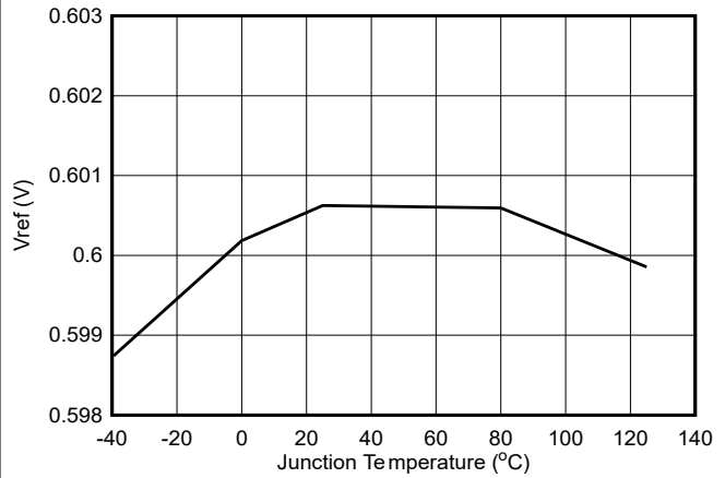
Figure 5-8. V_{REF} Voltage
