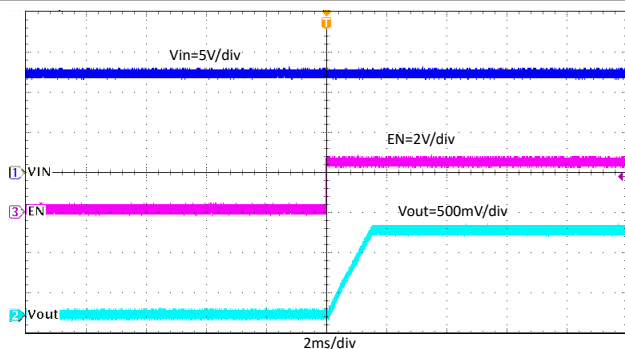
Figure 7-18. Start-up Through EN, I_{OUT} = 4A
