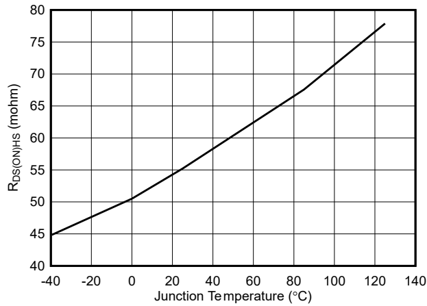
Figure 5-7. High-Side R_{DS(on)}
