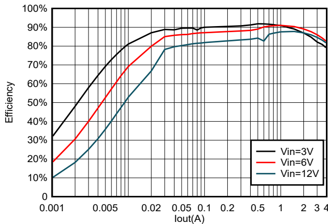
Figure 5-15. TPS564255B Efficiency at 1.05 V_{OUT} With a 1.5 \mu\text{H} Inductor
