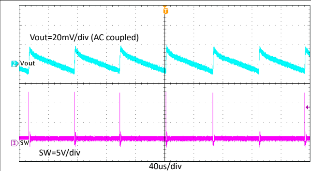
Figure 7-11. TPS564252B Output Voltage Ripple With 0.01A Loading
