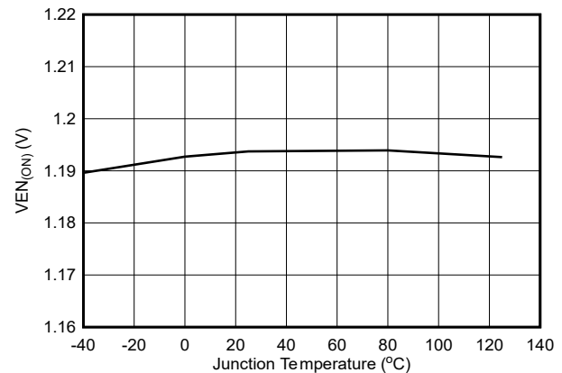
Figure 5-4. Enable On Threshold Voltage
