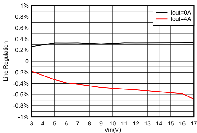
Figure 7-10. TPS564255B Line Regulation vs V_{IN}
