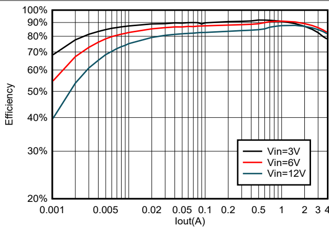
Figure 5-13. TPS564252B Efficiency at 1.05 V_{OUT} With a 1.5 \mu\text{H} Inductor
