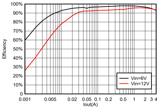
Figure 5-21. TPS564255B Efficiency at 5 V_{OUT} With a 4.7 \mu\text{H} Inductor
