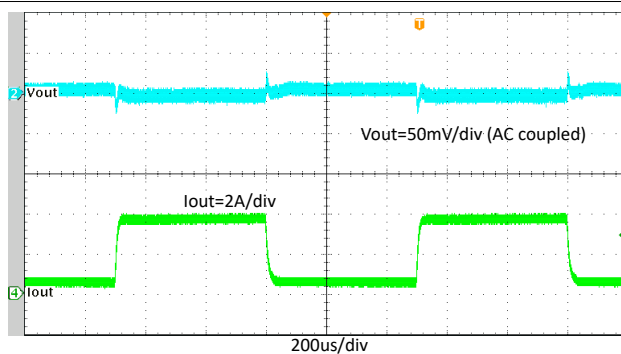
Figure 7-17. TPS564255B Transient Response With 0.4A to 3.6A
