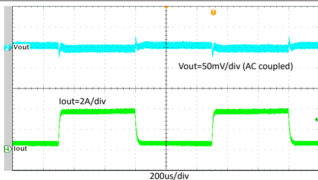
Figure 7-16. TPS564257B Transient Response With 0.4A to 3.6A
