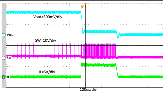
Figure 7-24. TPS564255B Normal Operation to Output Hard Short
