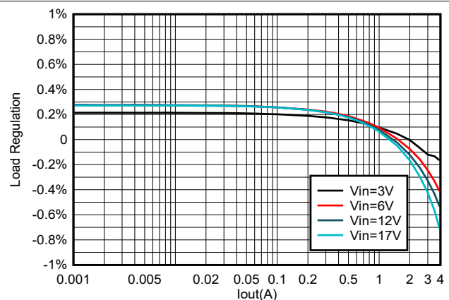
Figure 7-7. TPS564255B Load Regulation vs Loading
