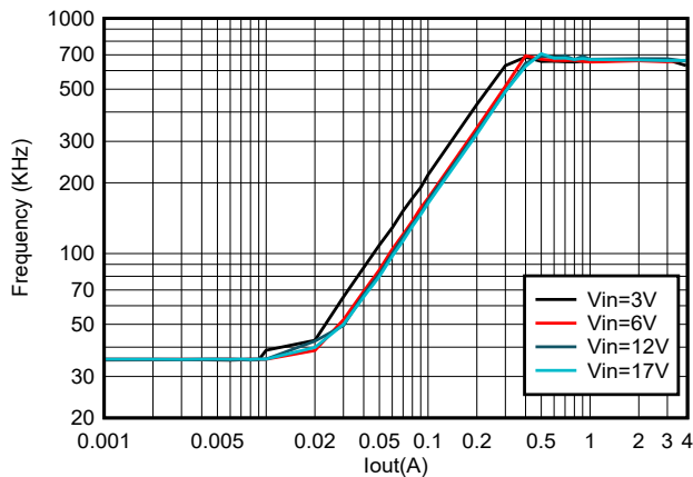
Figure 7-4. TPS564255B Frequency vs Loading
