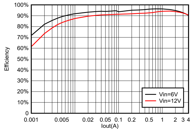
Figure 5-16. TPS564252B Efficiency at 3.3 V_{OUT} With a 3.3 \mu\text{H} Inductor
