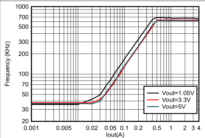
Figure 5-12. TPS564255B Frequency vs Loading, V_{IN} = 12\text{V}
