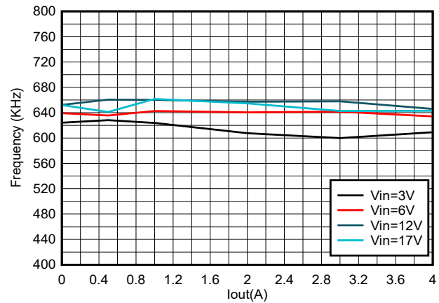
Figure 7-3. TPS564257B Frequency vs Loading
