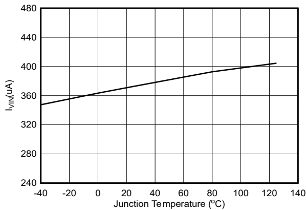
Figure 5-3. TPS564255B Quiescent Current
