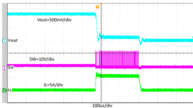
Figure 7-22. TPS564252B Normal Operation to Output Hard Short
