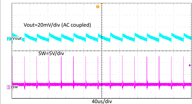
Figure 7-13. TPS564255B Output Voltage Ripple With 0.01A Loading
