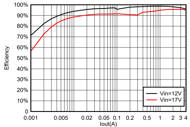
Figure 5-22. TPS564252B Efficiency at 10 V_{OUT} With a 6.8 \mu\text{H} Inductor
