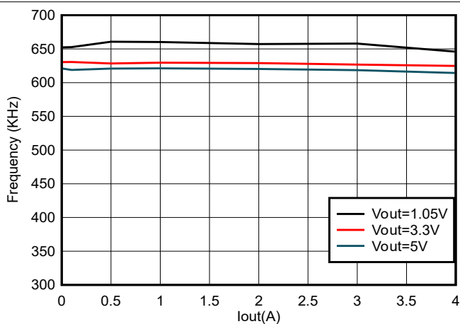
Figure 5-11. TPS564257B Frequency vs Loading, V_{IN} = 12\text{V}
