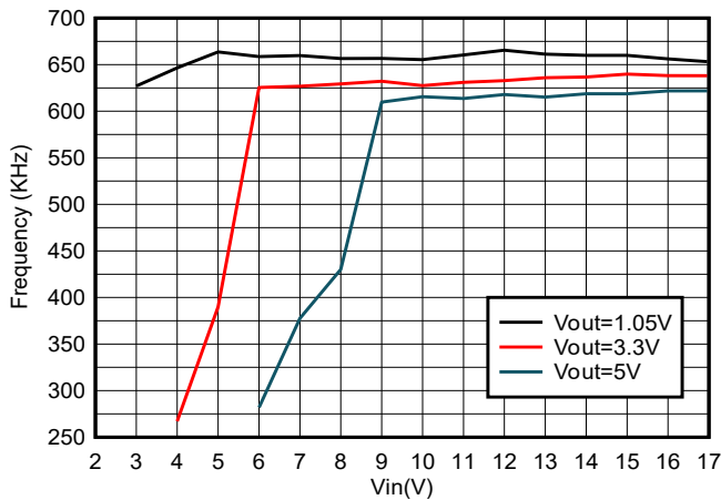
Figure 5-9. TPS564257B Frequency vs Input Voltage, I_{OUT} = 4\text{A}
