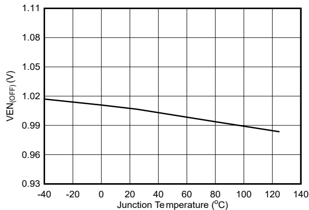
Figure 5-5. Enable Off Threshold Voltage
