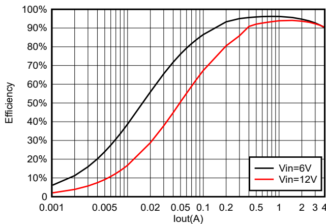
Figure 5-17. TPS564257B Efficiency at 3.3 V_{OUT} With a 3.3 \mu\text{H} Inductor
