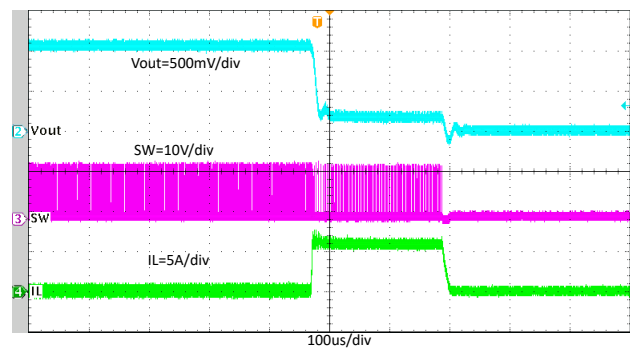
Figure 7-23. TPS564257B Normal Operation to Output Hard Short
