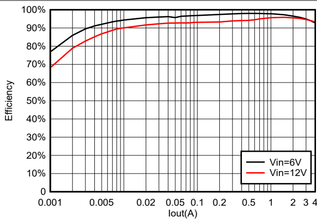
Figure 5-19. TPS564252B Efficiency at 5 V_{OUT} With a 4.7 \mu\text{H} Inductor
