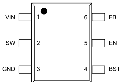
Figure 4-1. 6-Pin SOT563 DRL Package (Top View)
