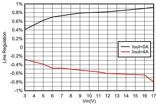
Figure 7-8. TPS564252B Line Regulation vs V_{IN}
