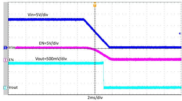
Figure 7-21. Shutdown With V_{IN} Falling, I_{OUT} = 4A
