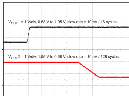
Figure 22. Voltage Change With I 2 C Control
