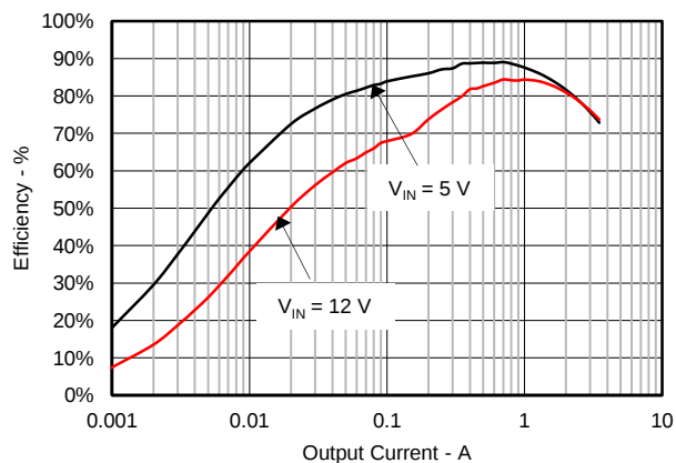
Figure 2. 1-V Efficiency, Eco-mode™
