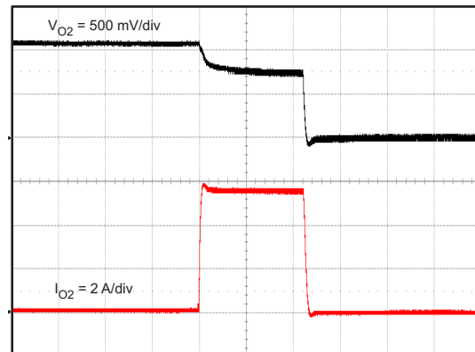
Figure 20. Overcurrent Protection, Buck 2
