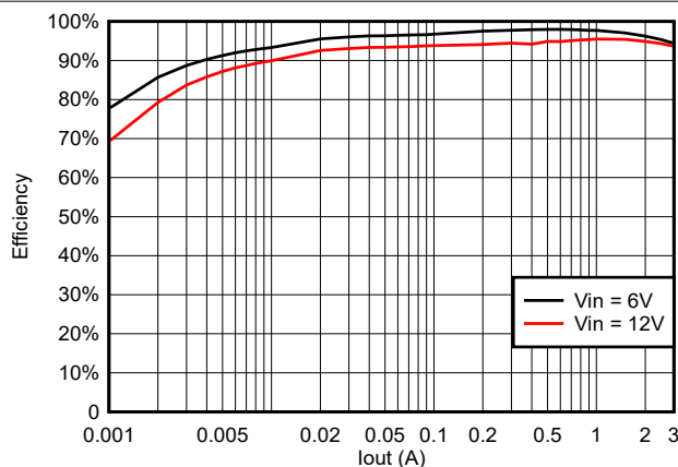
Figure 5-17. TPS563242 Efficiency at 5 V_{OUT} With a 2.2 \mu\text{H} Inductor
