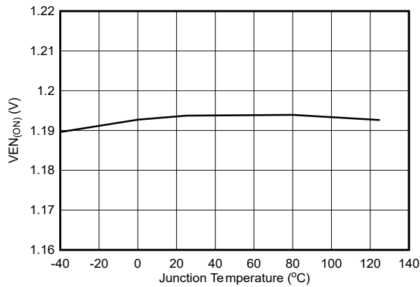
Figure 5-3. Enable On Threshold Voltage
