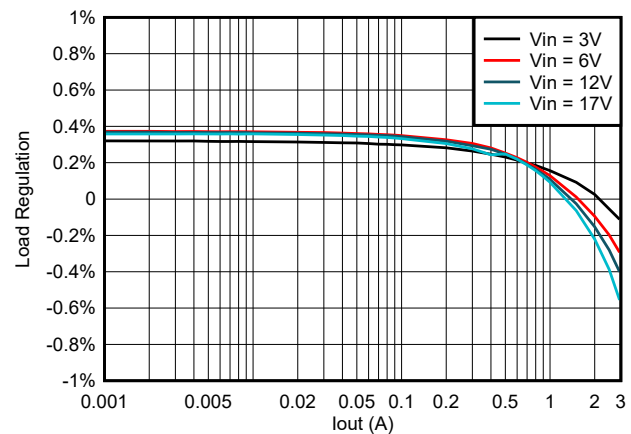
Figure 7-5. TPS563247 Load Regulation vs Loading
