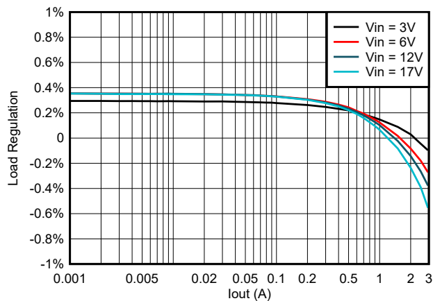
Figure 7-4. TPS563242 Load Regulation vs Loading
