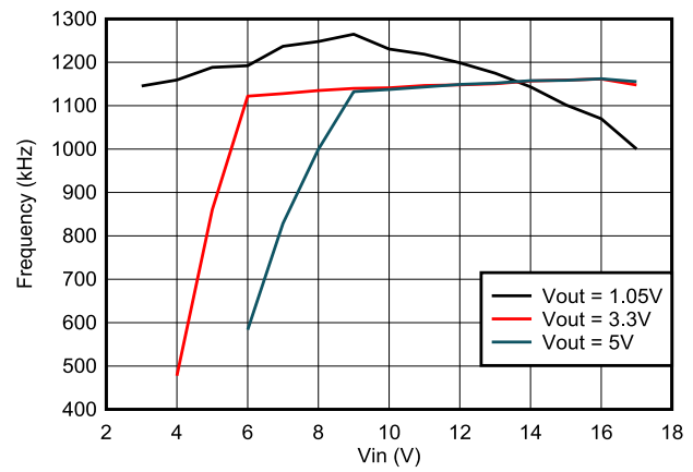
Figure 5-8. Frequency vs Input Voltage, I_{OUT} = 3\text{A}
