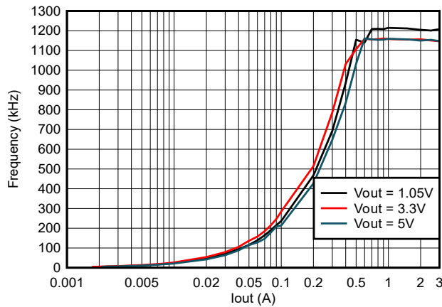
Figure 5-9. TPS563242 Frequency vs Loading, V_{IN} = 12\text{V}
