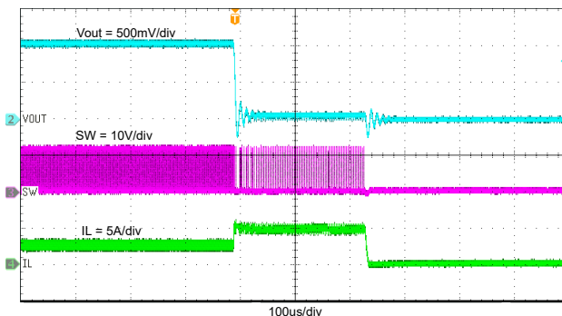
Figure 7-19. TPS563242 Normal Operation to Output Hard Short
