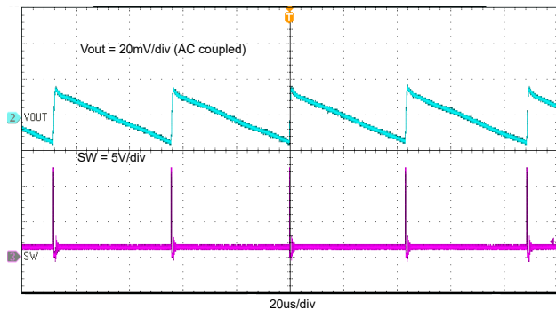
Figure 7-8. TPS563242 Output Voltage Ripple With 0.01A Loading
