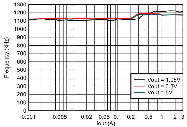
Figure 5-10. TPS563247 Frequency vs Loading, V_{IN} = 12\text{V}
