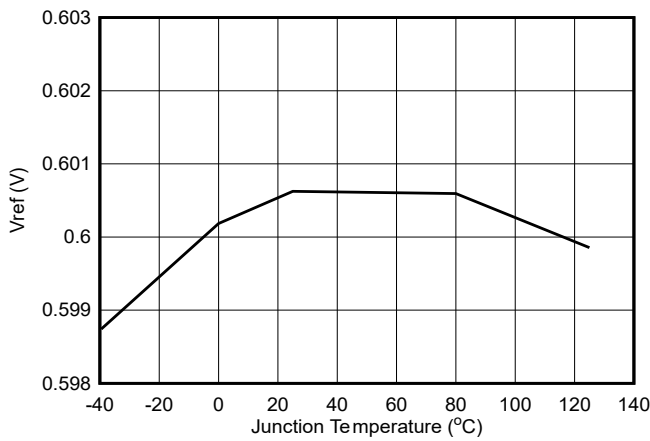
Figure 5-7. VREF Voltage
