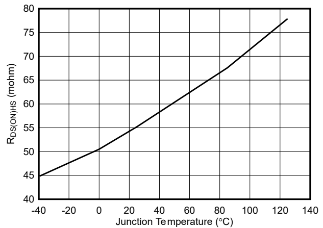
Figure 5-6. High-Side R_{DS(ON)}
