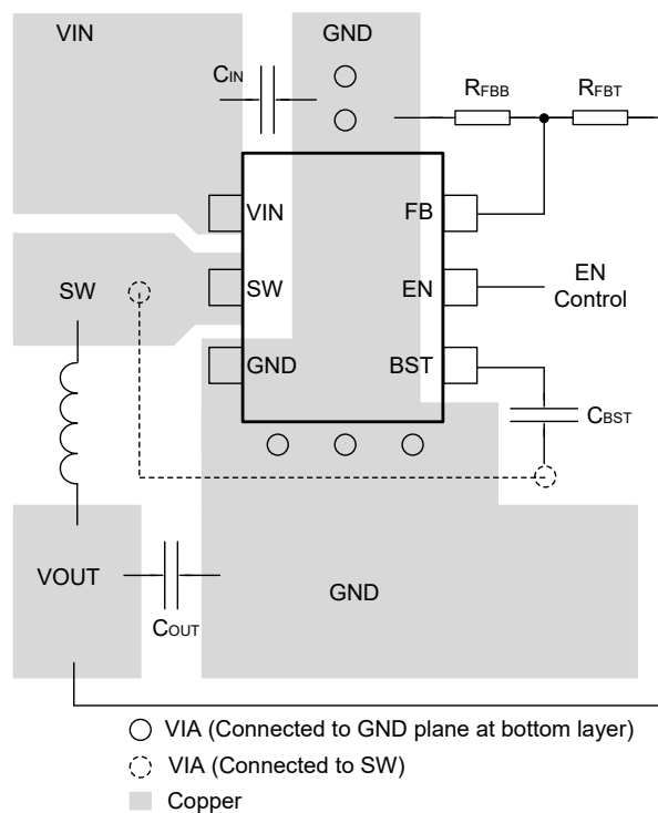
Figure 7-22. Suggested Layout
