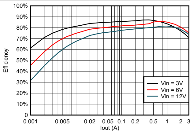
Figure 5-11. TPS563242 Efficiency at 0.6 V_{OUT} With a 0.68 \mu\text{H} Inductor
