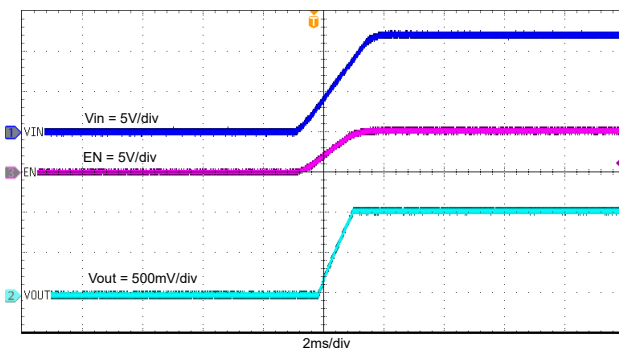
Figure 7-17. Start-up With V_{IN} Rising, I_{OUT} = 3A
