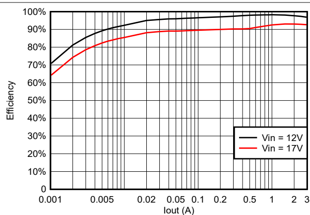
Figure 5-19. TPS563242 Efficiency at 10 V_{OUT} With a 4.7 \mu\text{H} Inductor
