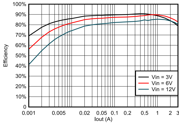
Figure 5-13. TPS563242 Efficiency at 1.05 V_{OUT} With a 0.82 \mu\text{H} Inductor
