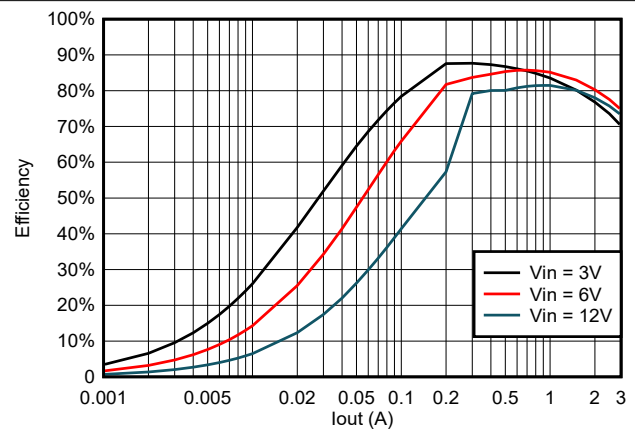
Figure 5-12. TPS563247 Efficiency at 0.6 V_{OUT} With a 0.68 \mu\text{H} Inductor
