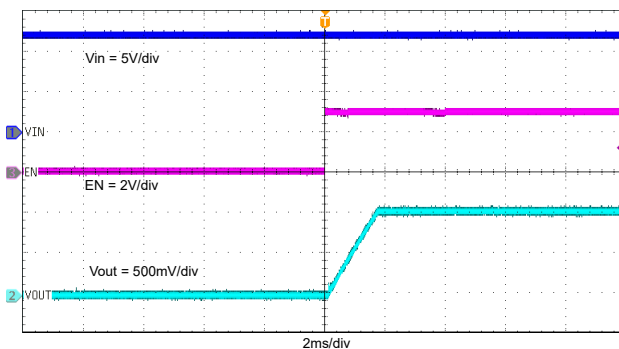
Figure 7-15. Start-up Through EN, I_{OUT} = 3A
