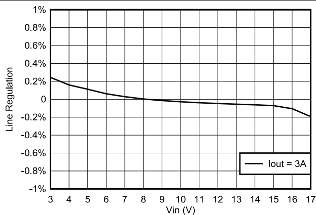
Figure 7-6. TPS563242 Line Regulation vs V_{IN}
