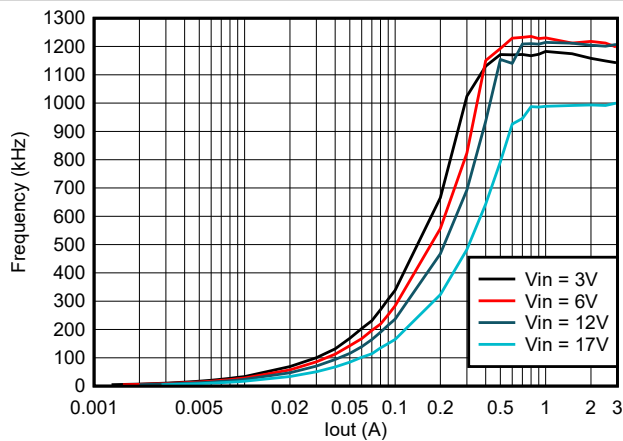
Figure 7-2. TPS563242 Frequency vs Loading
