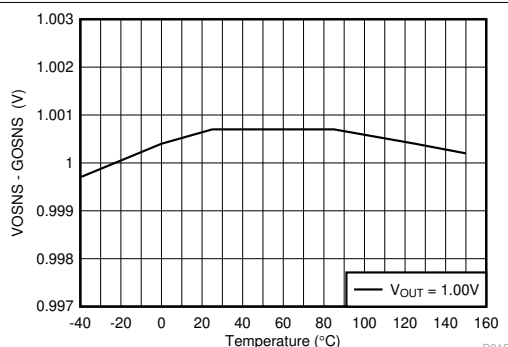
Figure 6-15. Output Voltage vs Junction Temperature V_{OUT\_COMMAND} = 1\text{ V}
