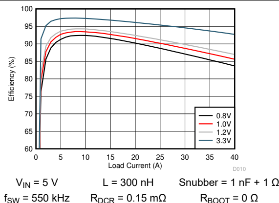
Figure 6-10. TPS546D24S Efficiency vs Output Current
