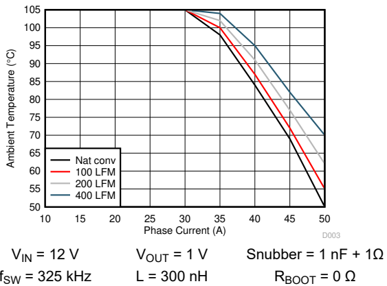
Figure 6-3. TPS546D24S Safe Operating Area
