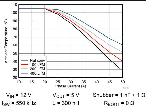
Figure 6-8. TPS546D24S Safe Operating Area
