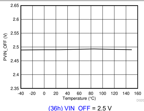
Figure 6-21. Turnoff Voltage vs Junction Temperature
