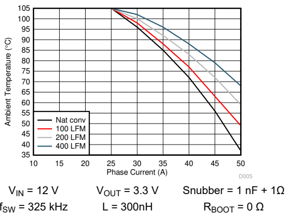
Figure 6-5. TPS546D24S Safe Operating Area
