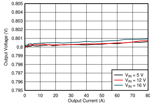
Figure 8-13. Load Regulation
