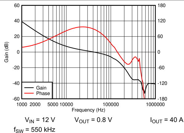
Figure 8-15. Total-Loop Bode Plot
