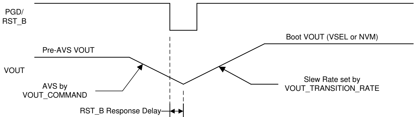
Figure 7-7. TPS546D24S Output Voltage Reset
