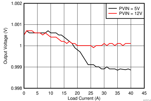
Figure 8-3. Load Regulation
