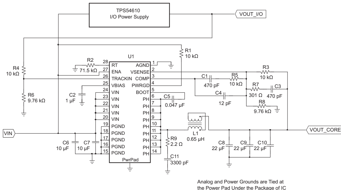
Figure 10. Application Circuit
