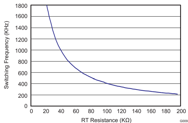
Figure 24. Switching Frequency vs RT Set Resistor
