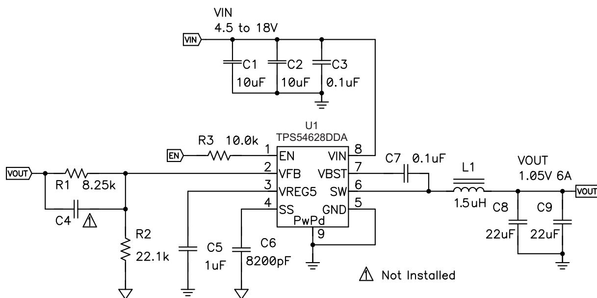
Figure 12. Simplified Application Schematic Example
