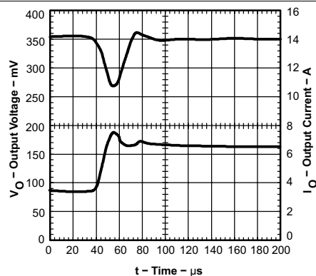
Figure 14. Transient Response
