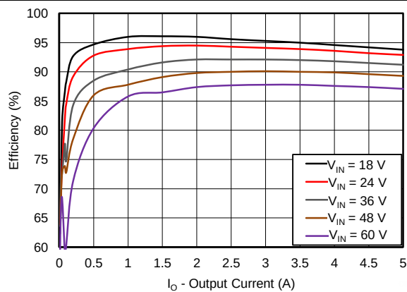
Figure 53. Efficiency vs Output Current
