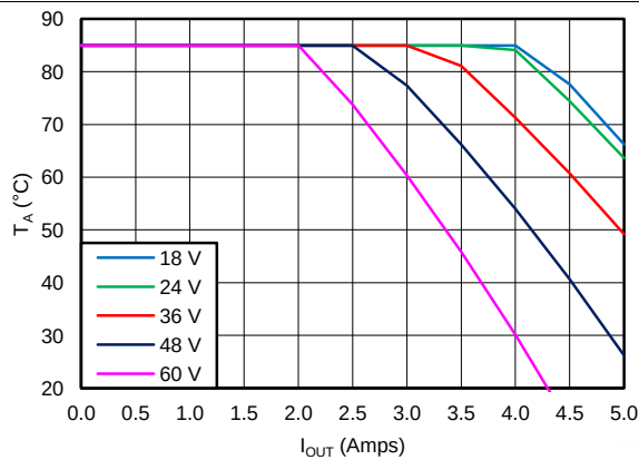
Figure 60. 12-V Outputs
