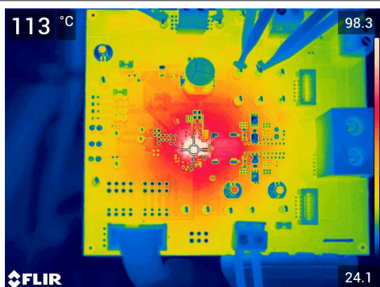
Figure 8-25. Thermal Characteristics, 1.2-MHz FCCM, Internal LDO, 35-A Load
