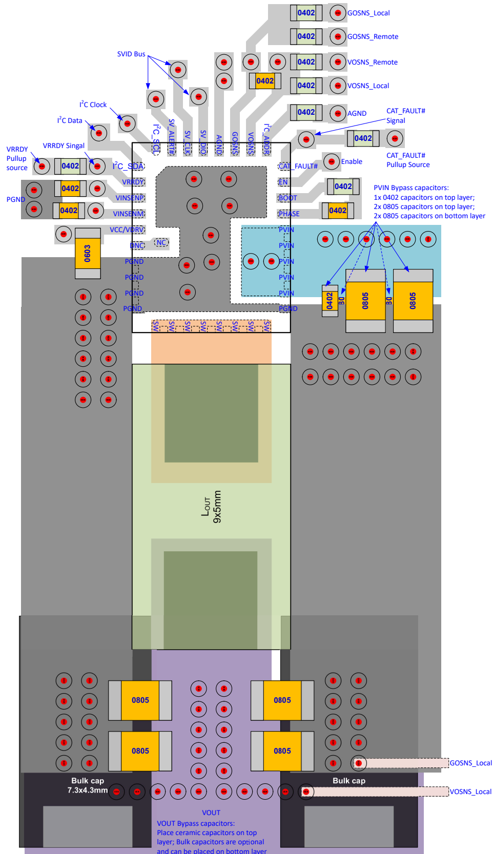
Figure 8-20. Layout Recommendation
