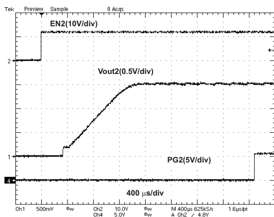
Figure 11. VO2=1.5V, PG2
