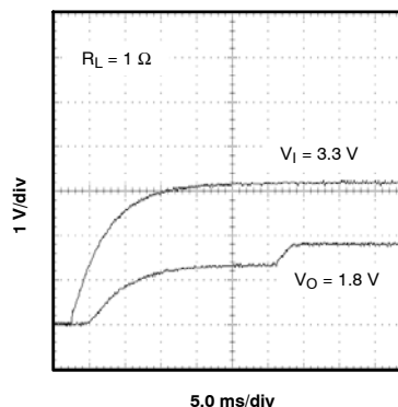
START-UP WAVEFORM
