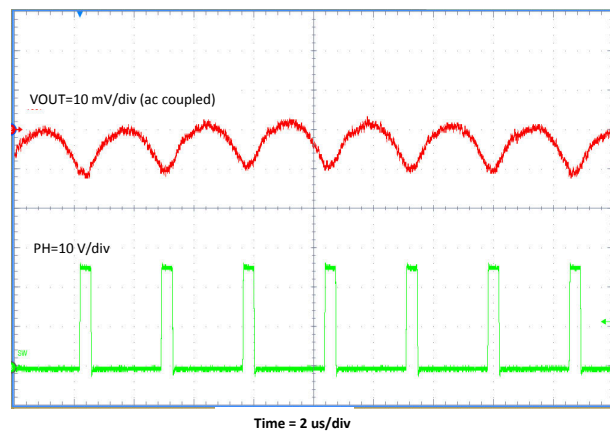
Figure 7-8. Output Voltage Ripple
