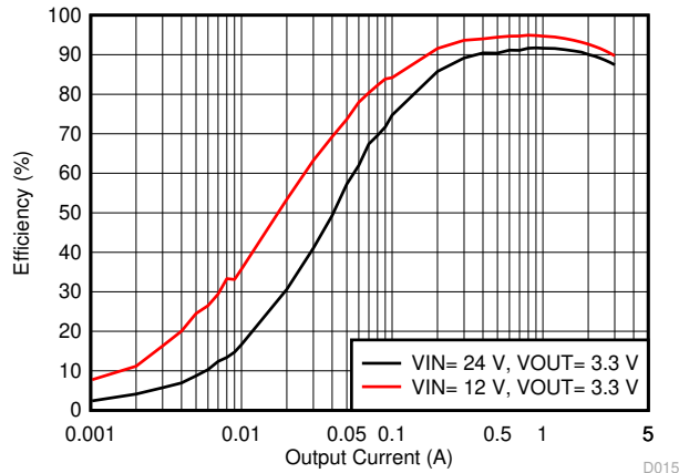
Figure 7-2. Efficiency
