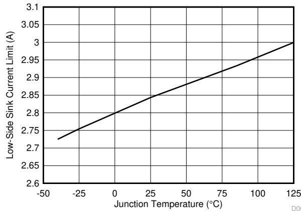
Figure 5-9. Low-Side Sink Current Limit Threshold vs Junction Temperature
