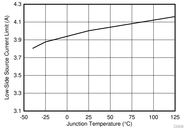
Figure 5-8. Low-Side Source Current Limit Threshold vs Junction Temperature
