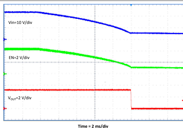
Figure 7-13. Shutdown Relative to VIN
