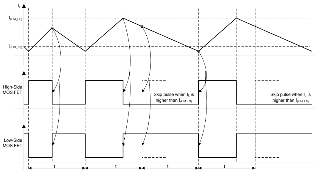
Figure 6-2. Overcurrent Protection for Both MOSFETs
