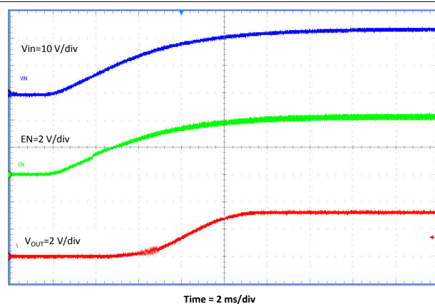
Figure 7-12. Start-Up Relative to VIN
