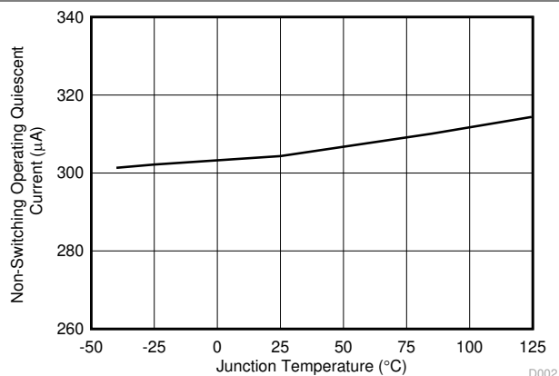
Figure 5-2. Non-Switching Operating Quiescent Current vs Junction Temperature
