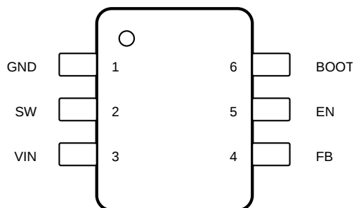
Figure 4-1. 6-Pin SOT-23-THN, DDC Package (Top View)
