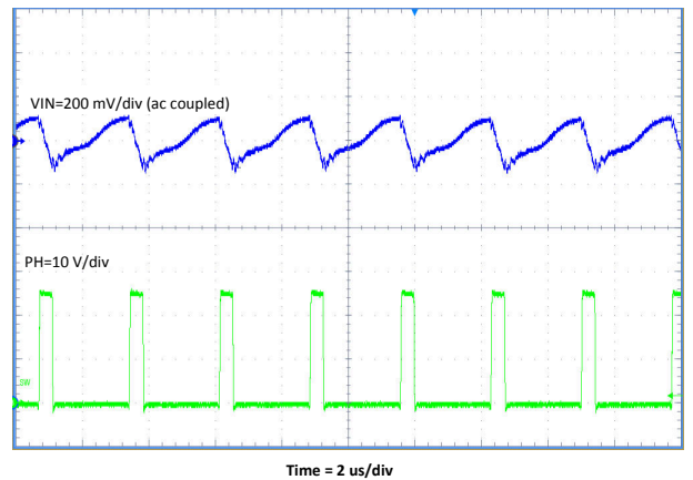
Figure 7-5. Input Voltage Ripple
