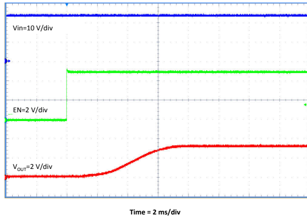
Figure 7-14. Start-Up Relative to EN
