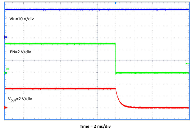
Figure 7-15. Shutdown Relative to EN
