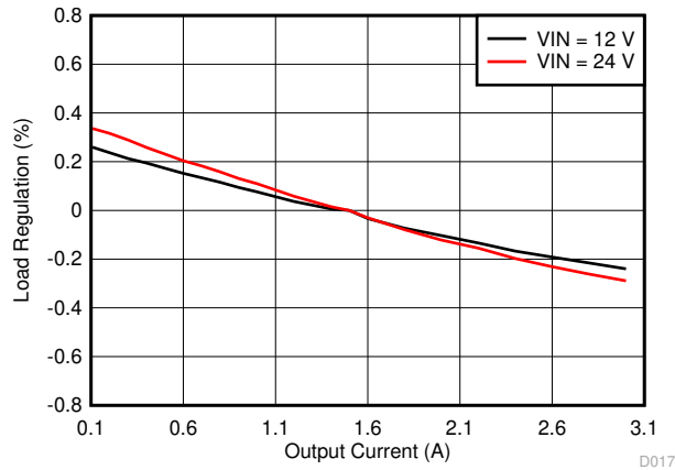
Figure 7-4. Load Regulation
