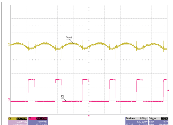
Figure 17. Output Ripple
