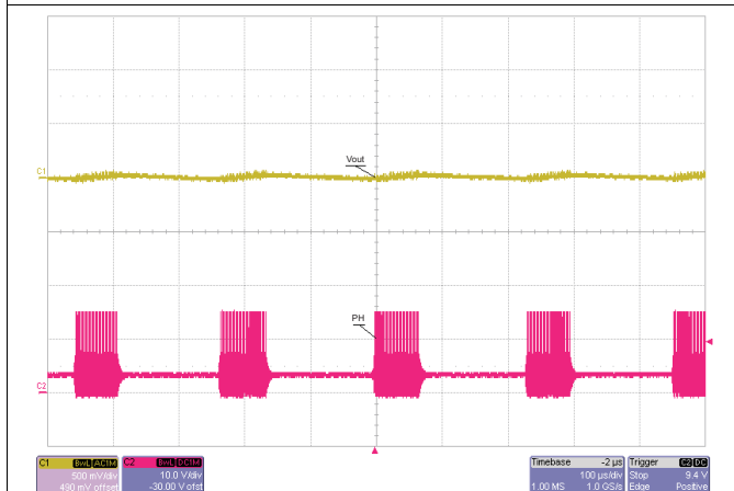
Figure 21. Eco-mode
