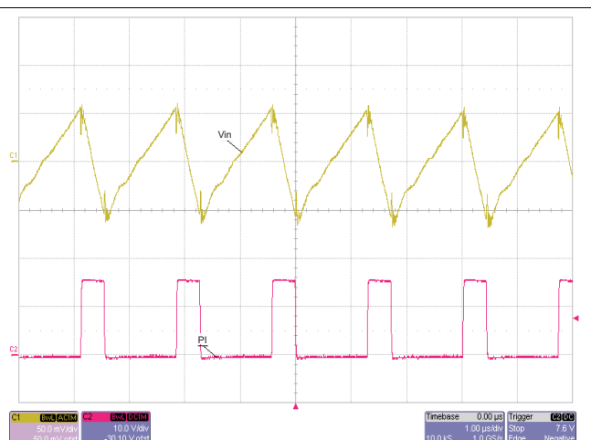
Figure 18. Input Ripple
