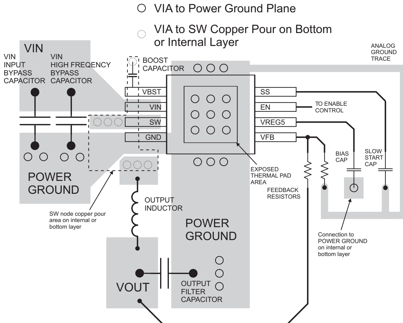
Figure 16. PCB Layout
