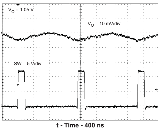
Figure 11. VOLTAGE RIPPLE AT OUTPUT ( I_O = 2\text{ A} )
