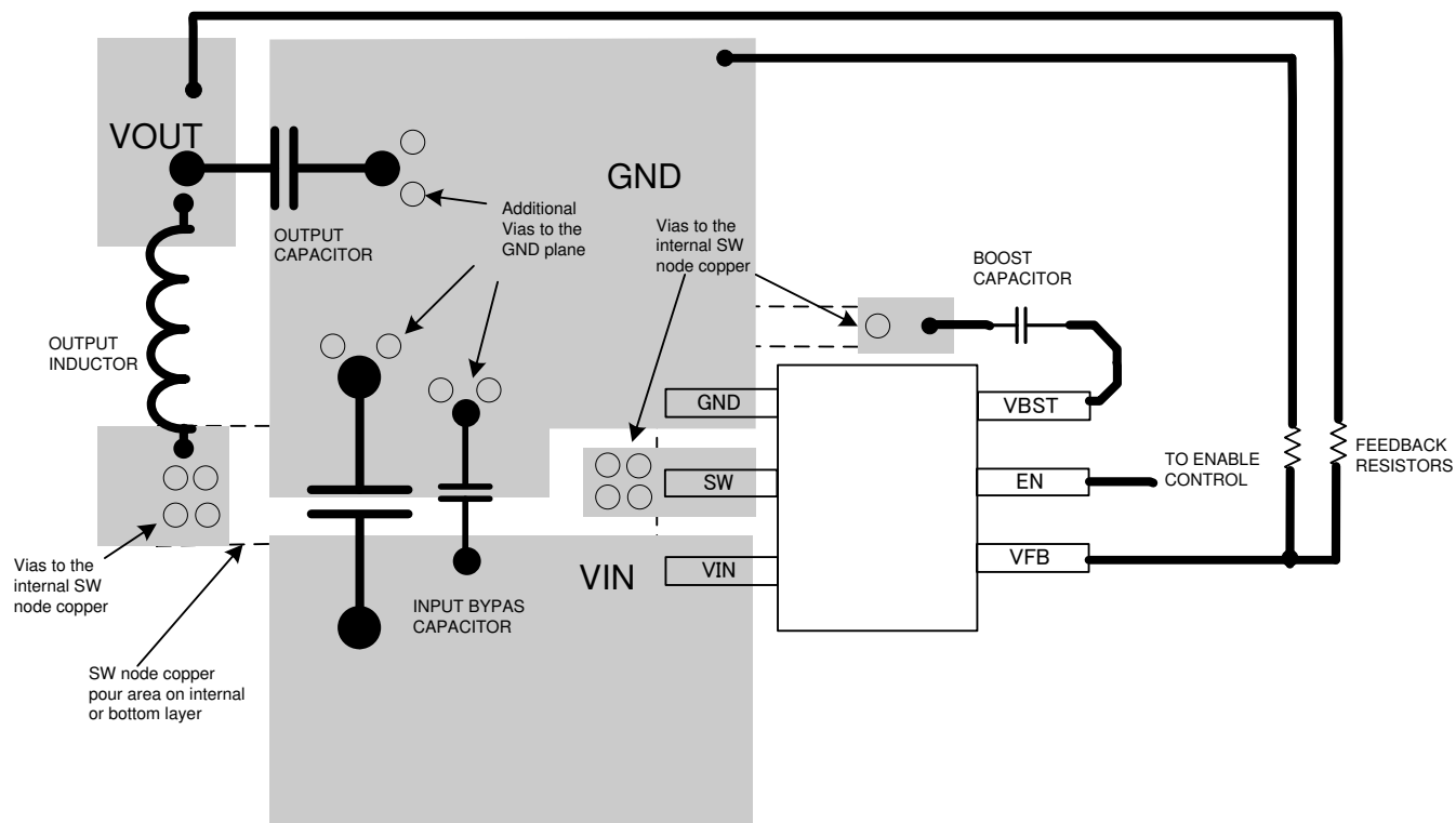
Figure 7-16. Board Layout
