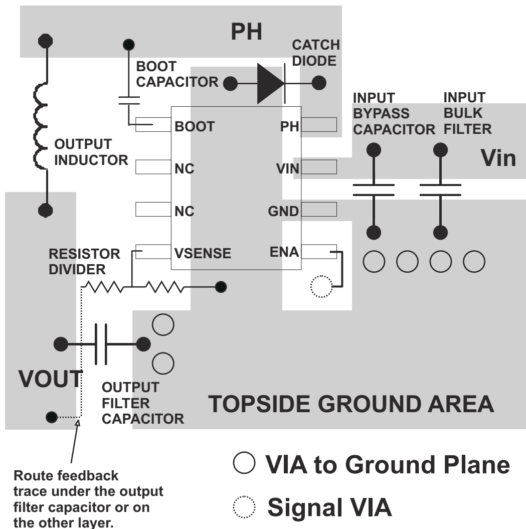
Figure 7-17. Design Layout
