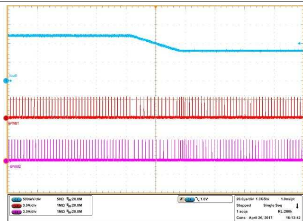
Figure 90. VOUTA VID-down Change
