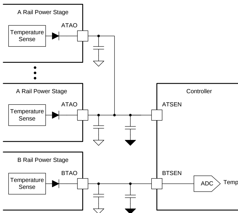
Figure 10. Temperature Sense
