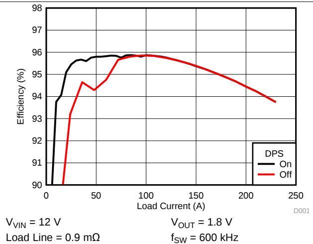
Figure 3. Efficiency
