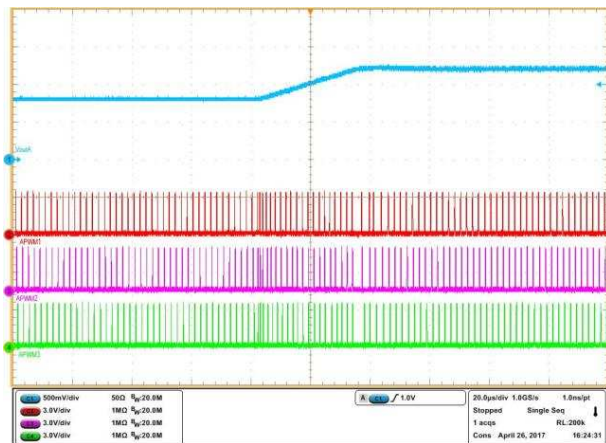
Figure 87. VOUTA Transient Response
