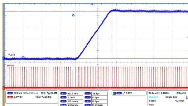
Figure 8-16. AVS transition up channel B
