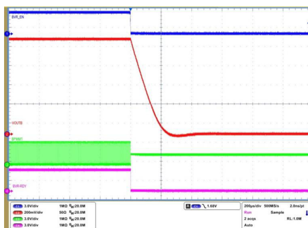
Figure 8-14. Shutdown (immediate off) channel B
