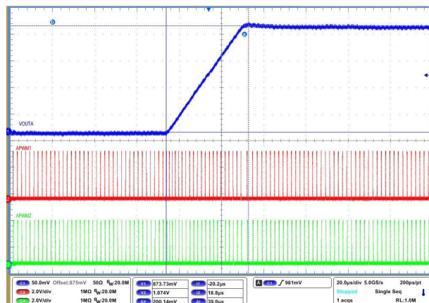
Figure 8-11. AVS up transition channel A
