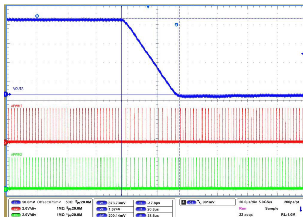
Figure 8-12. AVS down transition channel A
