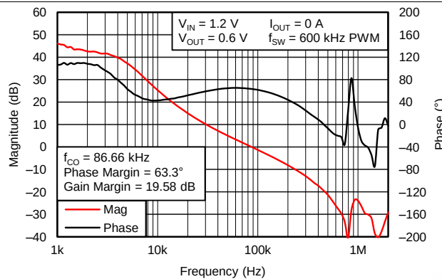
Figure 34. Bode Plot, No Load
