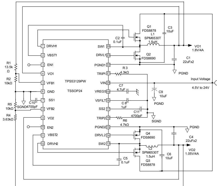
Figure 7. TSSOP
