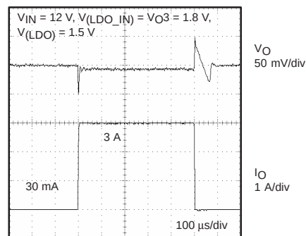
LDO LOAD TRANSIENT RESPONSE
