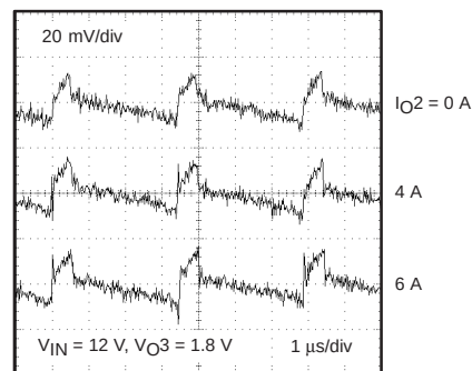
SBRC CH3 OUTPUT VOLTAGE RIPPLE
