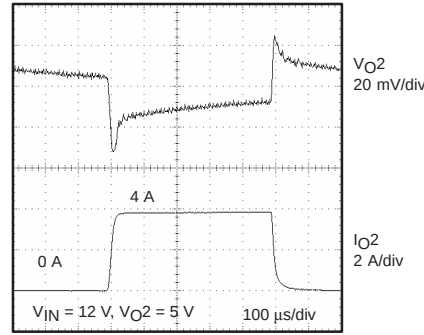
SBRC CH2 LOAD TRANSIENT RESPONSE
