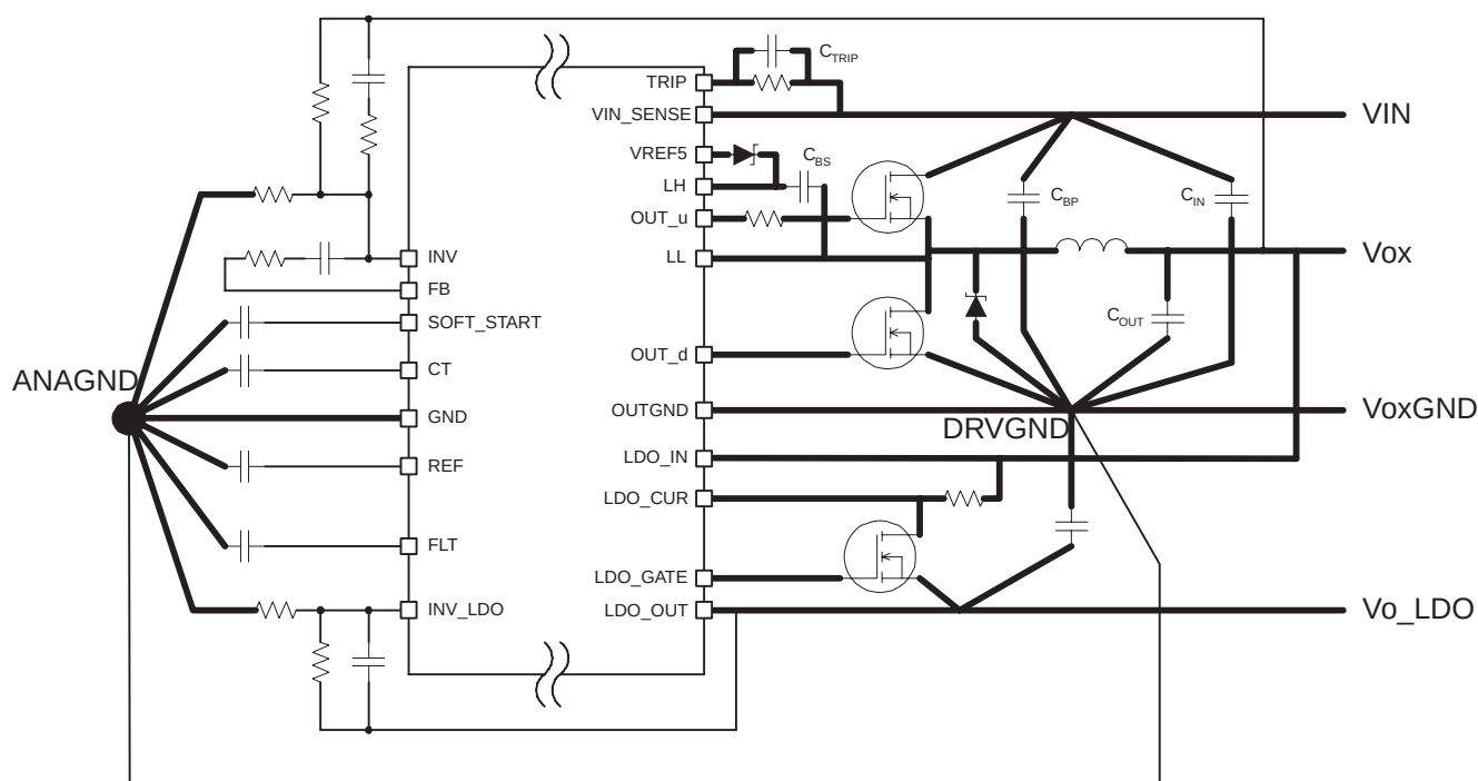
Figure 18. PCB Diagram
