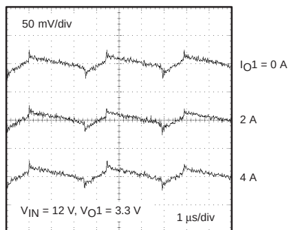
SBRC CH1 OUTPUT VOLTAGE RIPPLE
