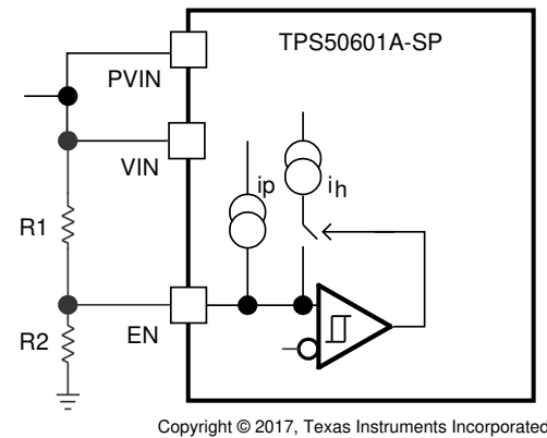
Figure 17. Adjustable VIN and PVIN UVLO
