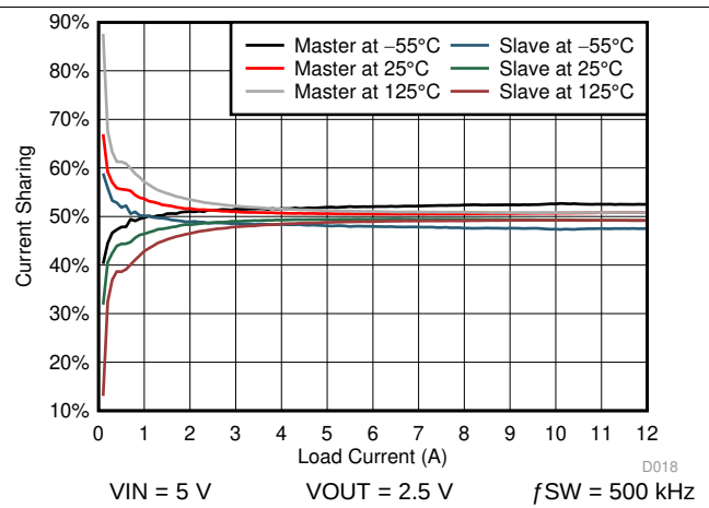
Figure 14. Current Sharing vs Load Current
