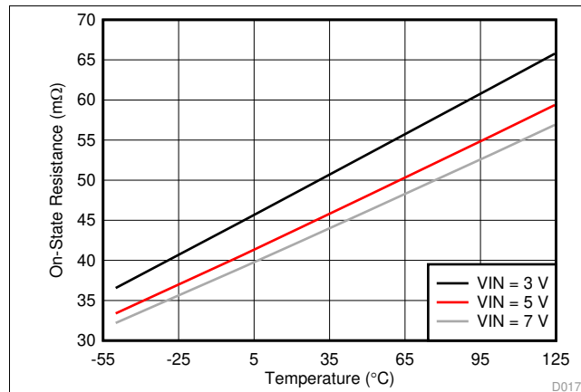
Figure 13. High-Side R_{DS(ON)} vs Temperature
