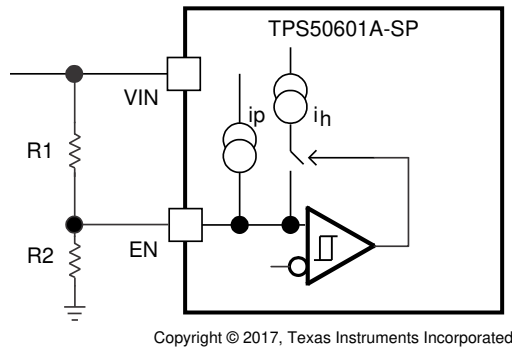
Figure 15. Adjustable VIN UVLO
