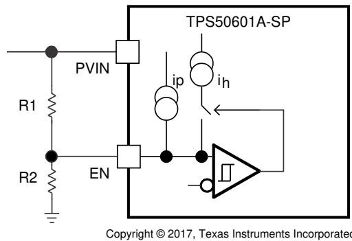
Figure 16. Adjustable PVIN UVLO
