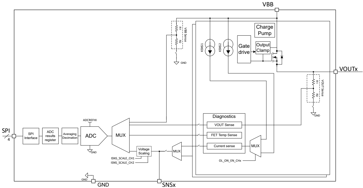
Figure 7-8. Integrated ADC Functional Block Diagram
