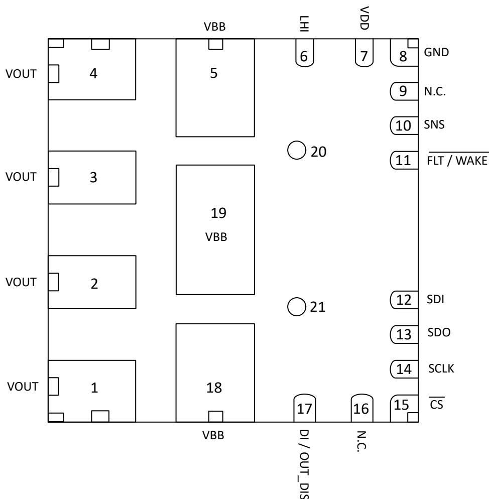
Figure 4-1. RBL Package, 21-Pin QFN-HR (Bottom View) - TPS481HS04-Q1
