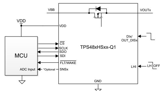
Application Circuit
