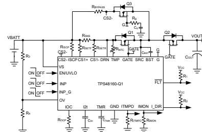
TPS48160-Q1 Application Circuit With Bulk Capacitor Charging
