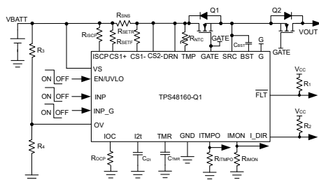
TPS48160-Q1 Application Circuit Driving Back to Back FETs
