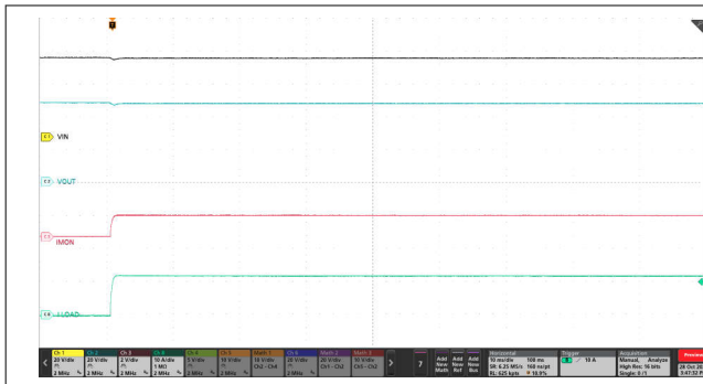
Figure 9-8. TPS4816-Q1 Current Monitoring Output (IMON) Transient Response
