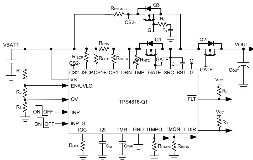
Figure 9-1. Driving Capacitive Load with TPS4816-Q1
