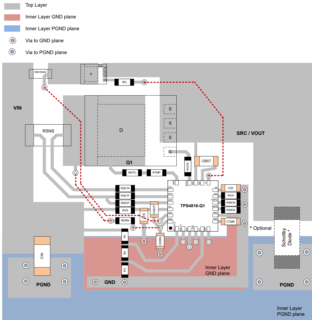
Figure 9-14. Typical PCB Layout Example of TPS4816-Q1
