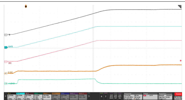
Figure 9-11. Inrush Current Profile With 1000µF at the Output (INP_G = High, INP = Low)
