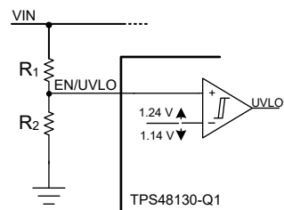
Figure 7-11. Programming Undervoltage Protection Threshold
