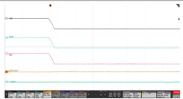
Figure 9-15. GATE Turn-OFF During Input Reverse Battery Fault
