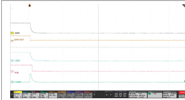
Figure 9-12. Output Short-Circuit Response of TPS4812-Q1
