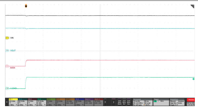
Figure 9-13. TPS4812-Q1 Current Monitoring Output (IMON) Transient Response
