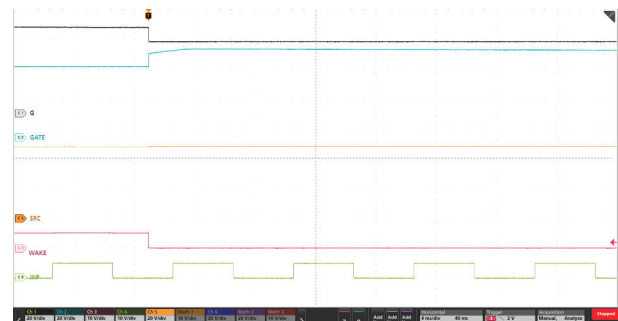
Figure 9-5. When \overline{\text{LPM}} = Low in LOAD WAKEUP state, \text{INP} Has No Control on \text{GATE}
