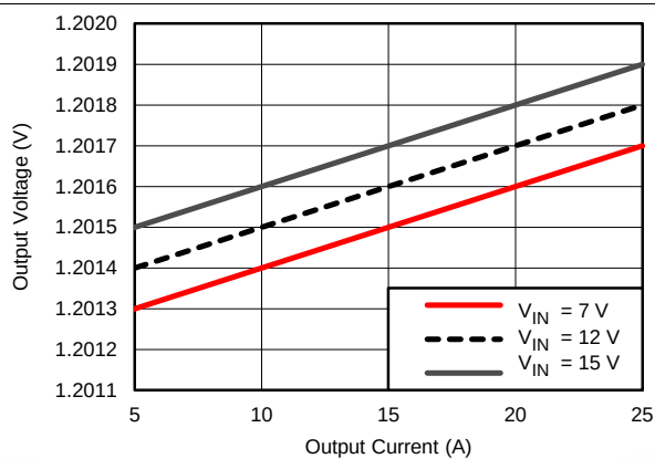
Figure 25. Load Regulation
