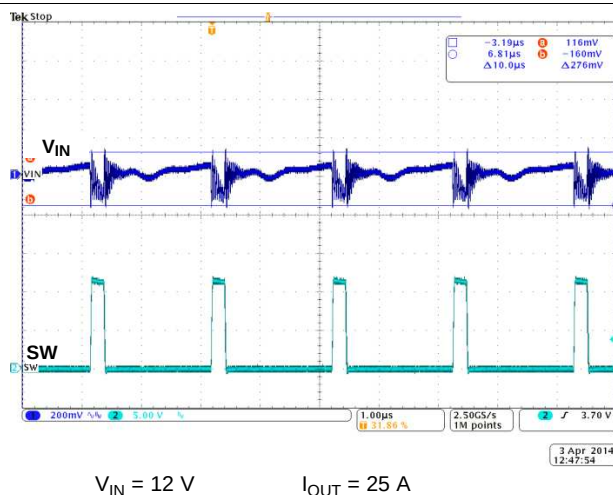
Figure 27. Input Voltage Ripple
