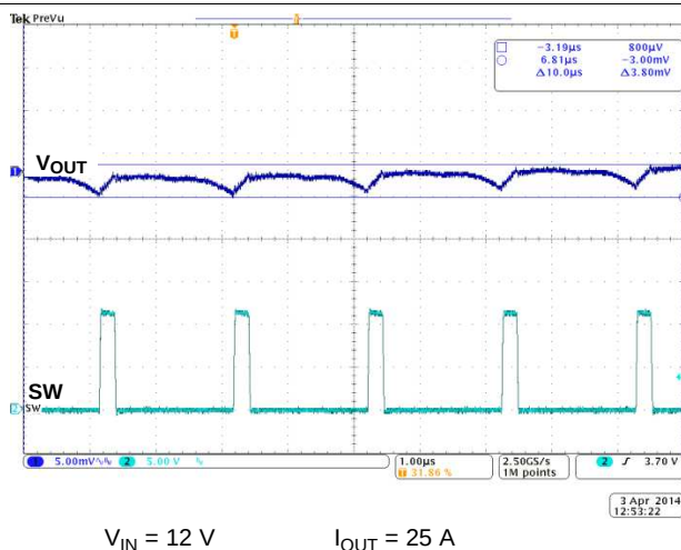
Figure 26. Output Voltage Ripple
