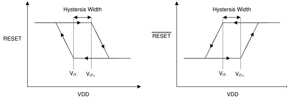
Figure 6-1. Hysteresis Diagram
