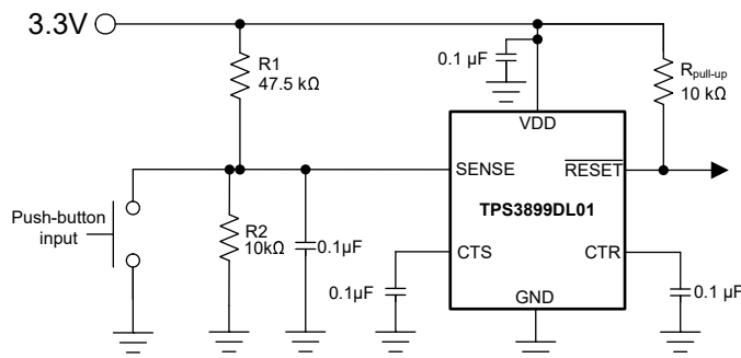
Figure 7-1. Design 1 - Adjustable Voltage Supervisor with Push-Button Functionality Circuit
