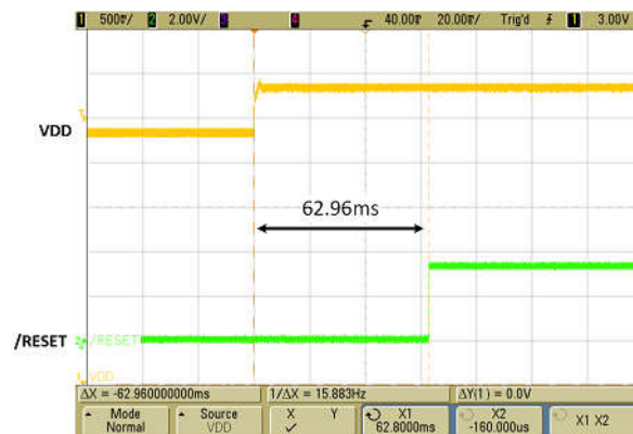
Figure 7-4. Reset Delay
