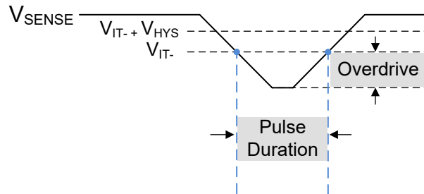
Figure 6-4. Overdrive vs Pulse Duration
