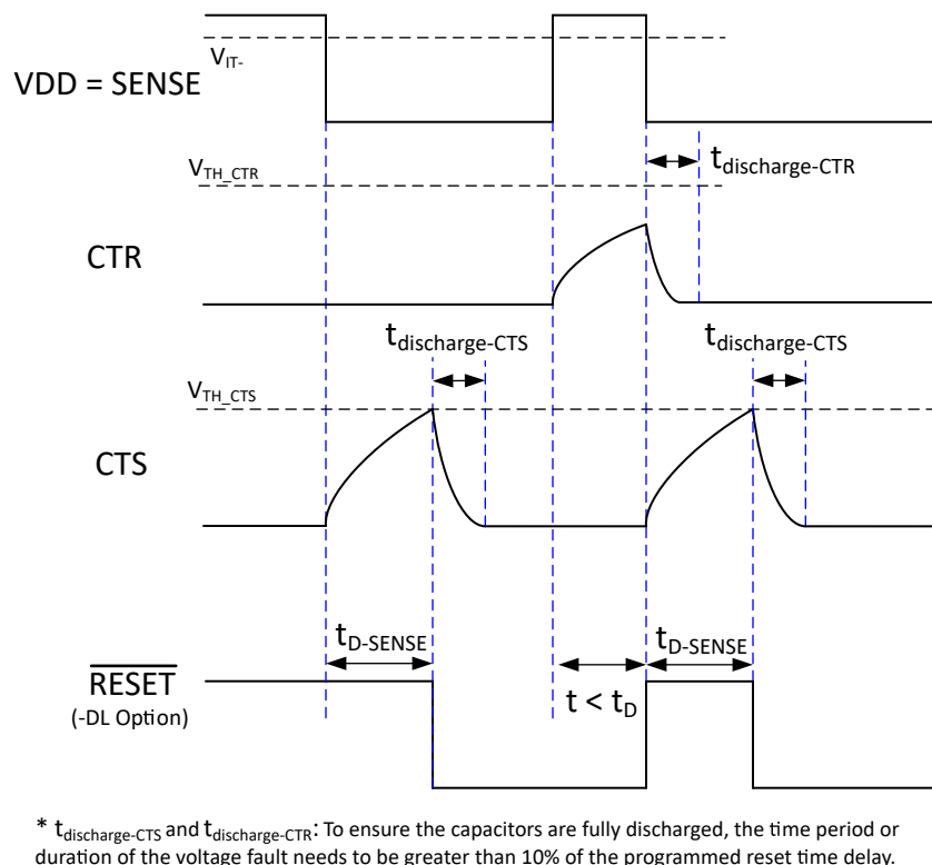
Figure 6-3. CTS and CTR Charge and Discharge Behavior Relative to VDD, SENSE and \overline{\text{RESET}}
