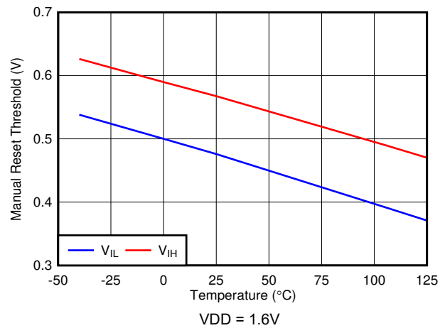
Figure 5-4. \overline{\text{MR}} Threshold vs Temperature
