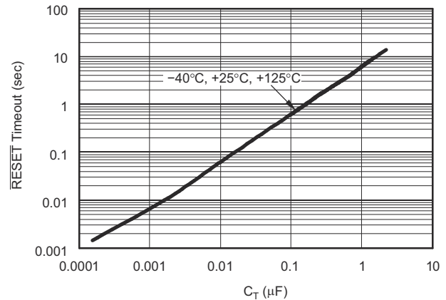
Figure 6-3. RESET Time-Out Period vs C_T
