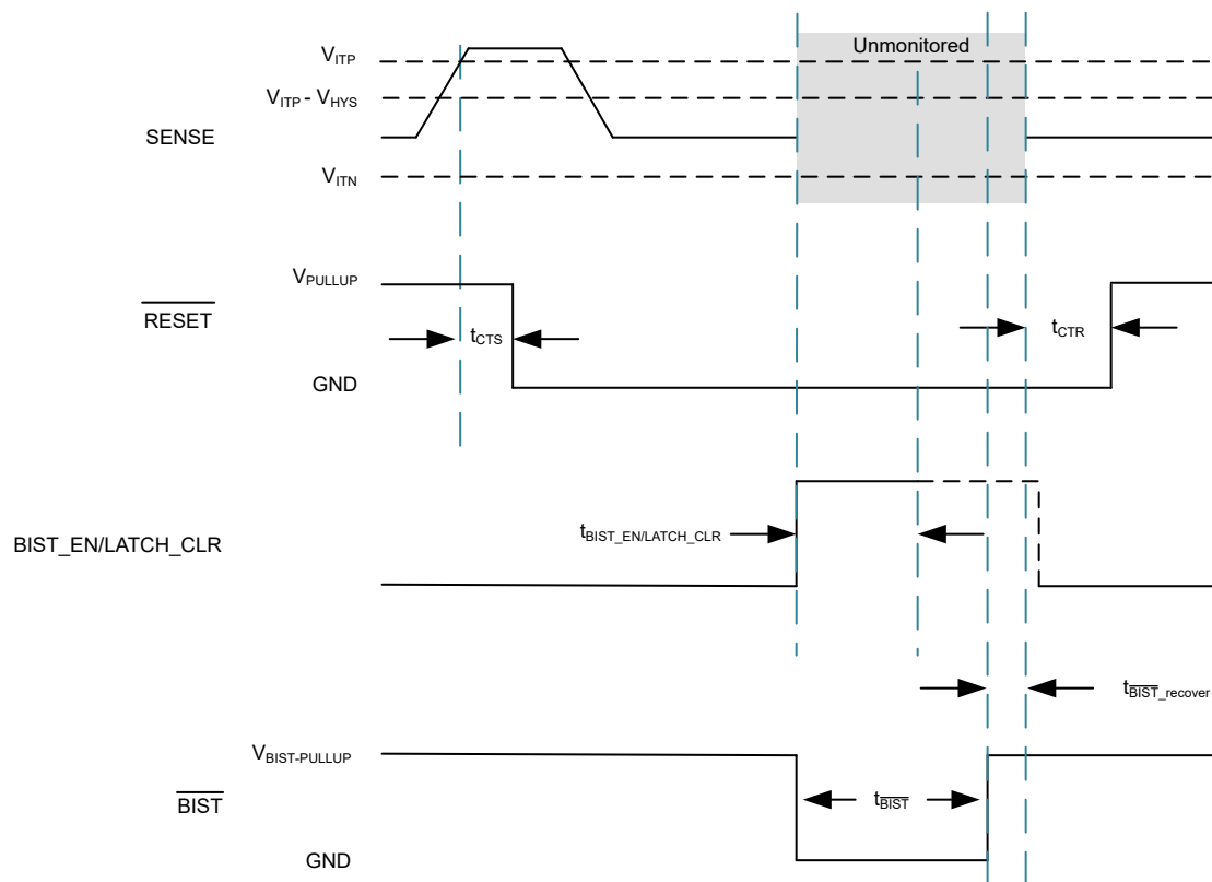
Figure 7-6. RESET Latch & Unlatch
