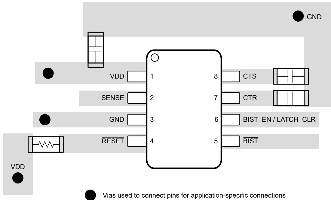
Figure 8-6. TPS3762 Recommended Layout
