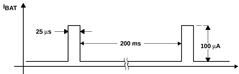
Figure 1. BATTOK Timing
