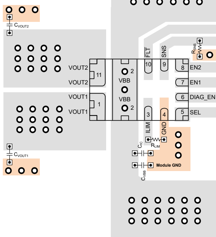
Figure 9-12. Layout Example without a GND Network
