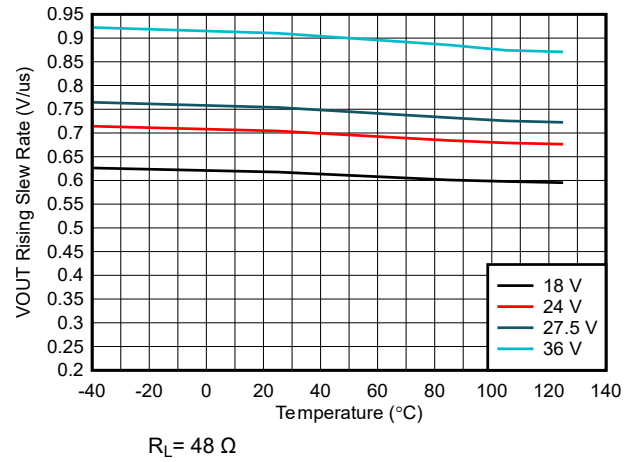
Figure 6-14. VOUT Rising Slew Rate ( SR_R ) vs Temperature vs VS Voltage
