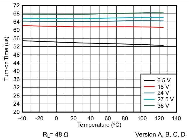
Figure 6-10. Turn-on Time ( t_{ON} ) vs Temperature vs VS Voltage
