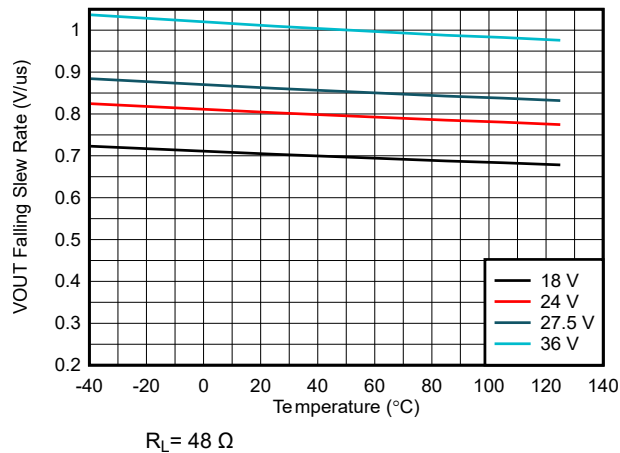
Figure 6-15. VOUT Falling Slew Rate ( SR_F ) vs Temperature vs VS Voltage
