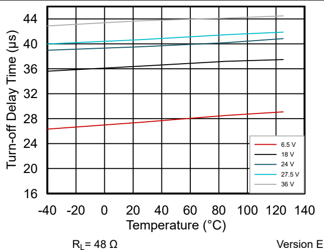
Figure 6-9. Turn-off Delay Time ( t_{DF} ) vs Temperature vs VS Voltage
