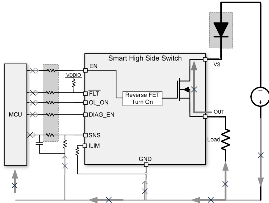
Figure 8-17. Reverse Protection With Blocking Diode
