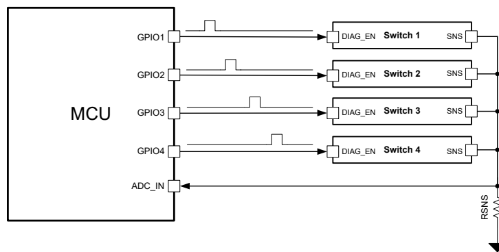
Figure 8-20. Resistor sharing
