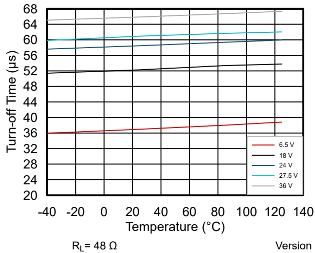
Figure 6-13. Turn-off Time ( t_{OFF} ) vs Temperature vs VS Voltage
