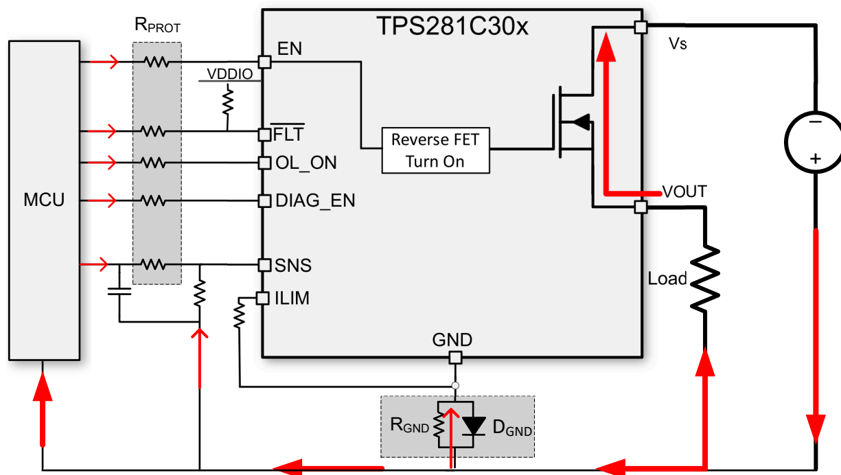
Figure 8-19. MCU IO Protections
