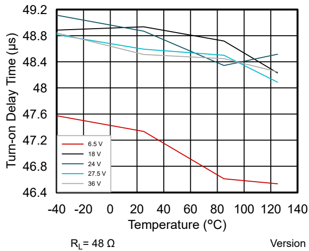
Figure 6-7. Turn-on Delay Time ( t_{DR} ) vs Temperature vs VS Voltage
