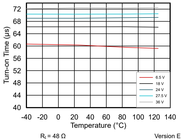
Figure 6-11. Turn-on Time ( t_{ON} ) vs Temperature vs VS Voltage
