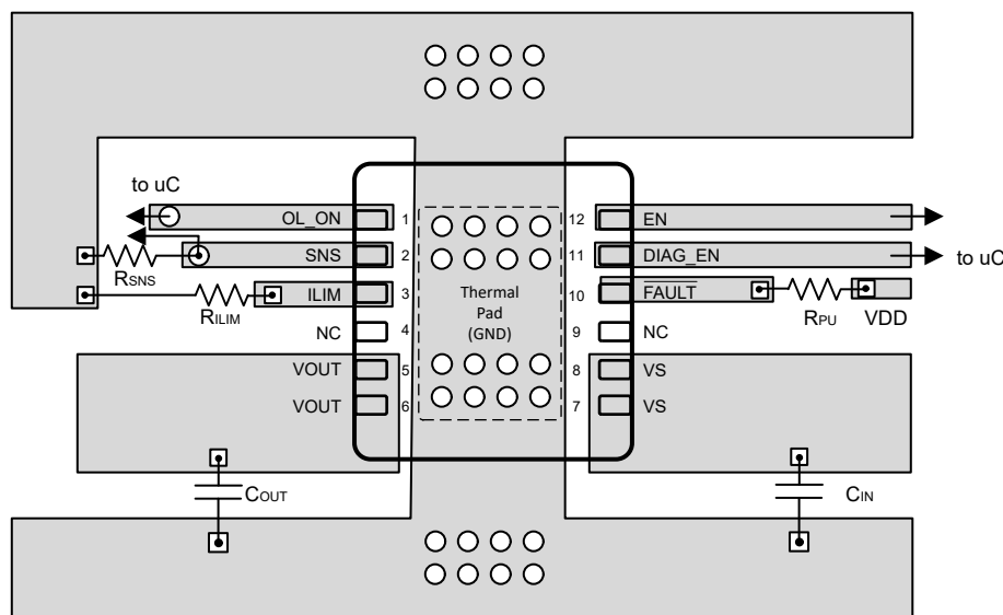
Figure 9-2. DNT Layout Without a GND Network
