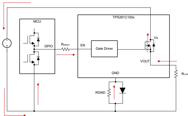
Figure 8-19. MCU IO Protections
