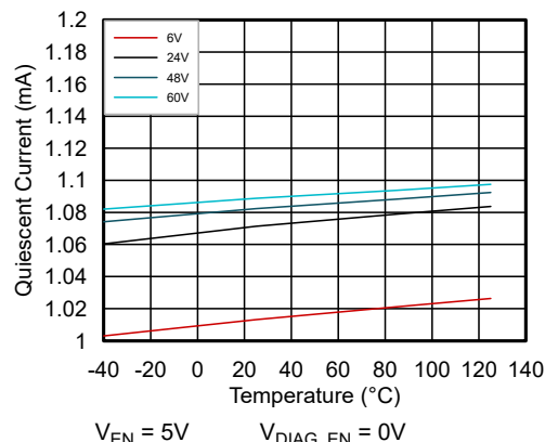
Figure 6-2. Quiescent Current ( I_{Q, VS} ) From VS Input Supply vs Temperature vs VS Voltage
