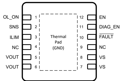
Figure 5-1. DNT Package, 12-Pin WSON (Top View)
