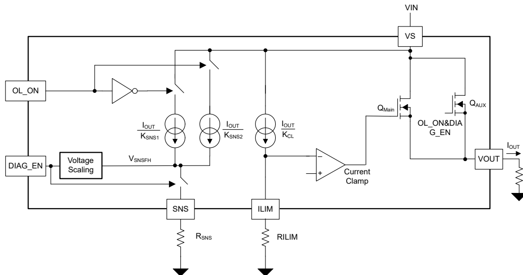
Figure 8-3. Current-Sense and Current-Limit Block Diagram
