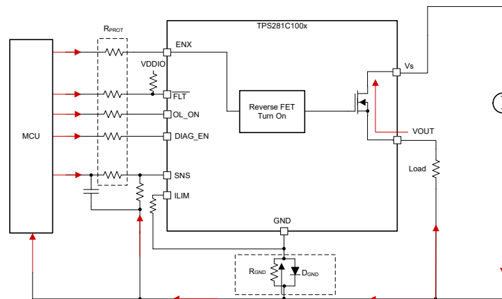
Figure 8-18. Reverse Protection With GND Network
