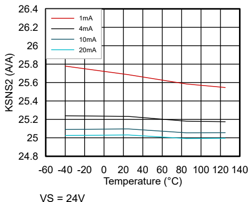
Figure 6-9. Current Sense Ratio ( KSNS_2 ) vs Temperature vs Load Current
