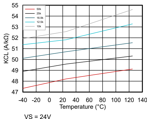
Figure 6-10. Current Limit Ratio ( K_{CL} ) vs Temperature vs R_{ILIM}
