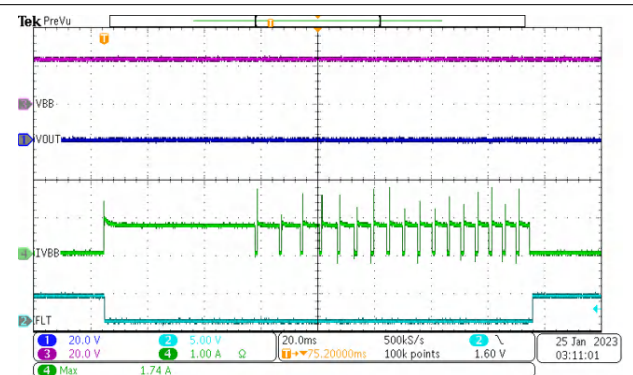
Figure 9-3. Enable into Short Circuit
