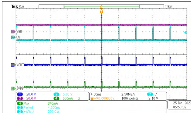
Figure 9-2. 250-kHz PWM Switching
